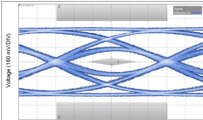
Figure 23. 25.78125 Gbps CAUI-4 Eye Mask with 10 in input channel and minimal output channel
