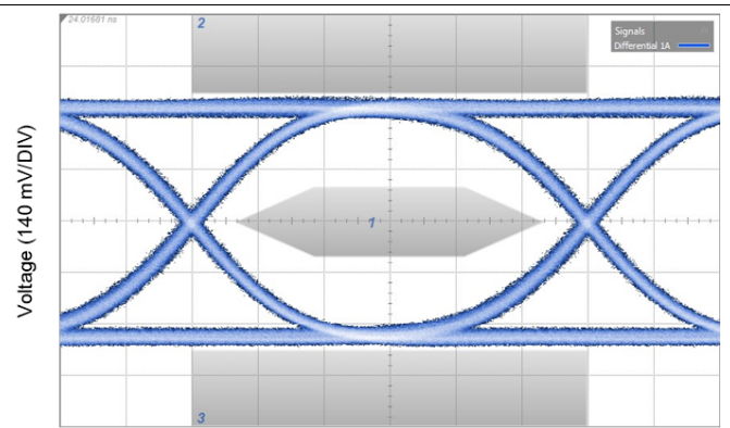
Figure 24. 10.3125 Gbps nPPI Eye Mask with 10 in input channel and minimal output channel
