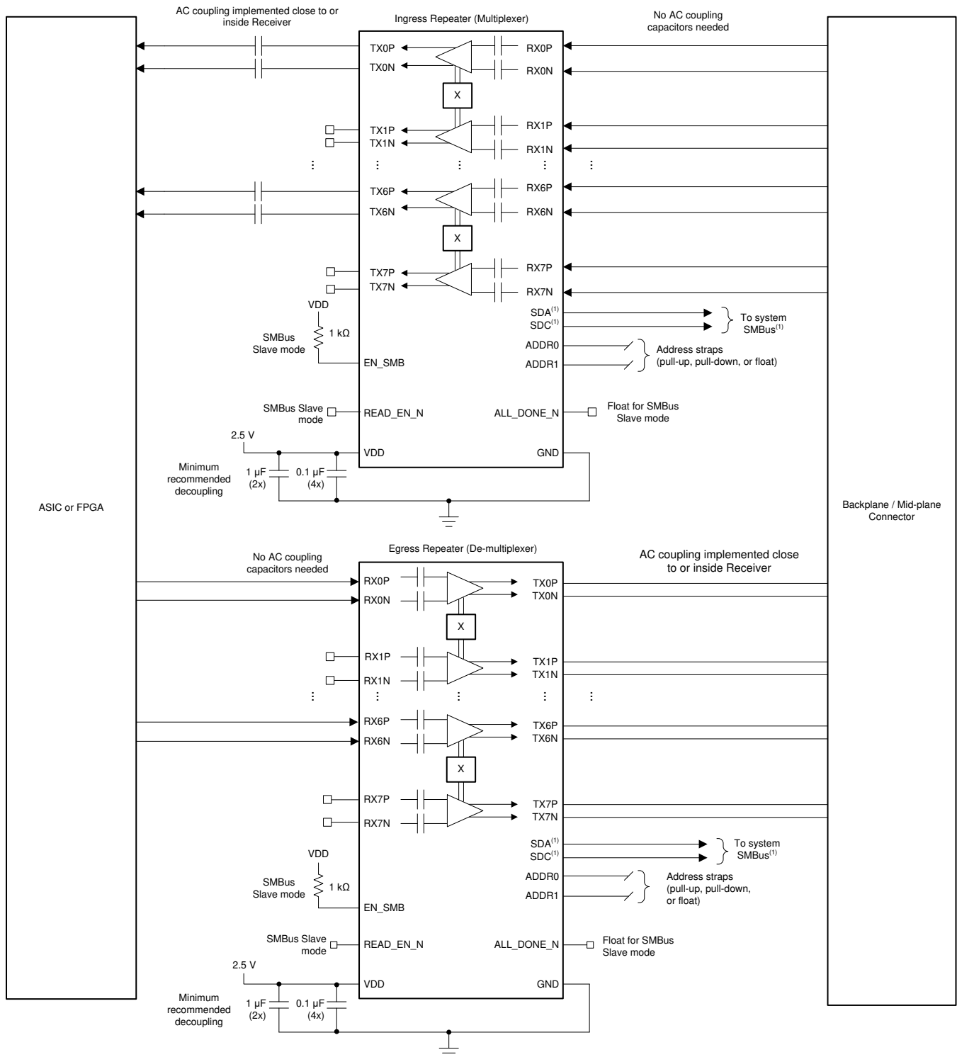
Figure 10. Typical backplane and mid-plane simplified schematic
