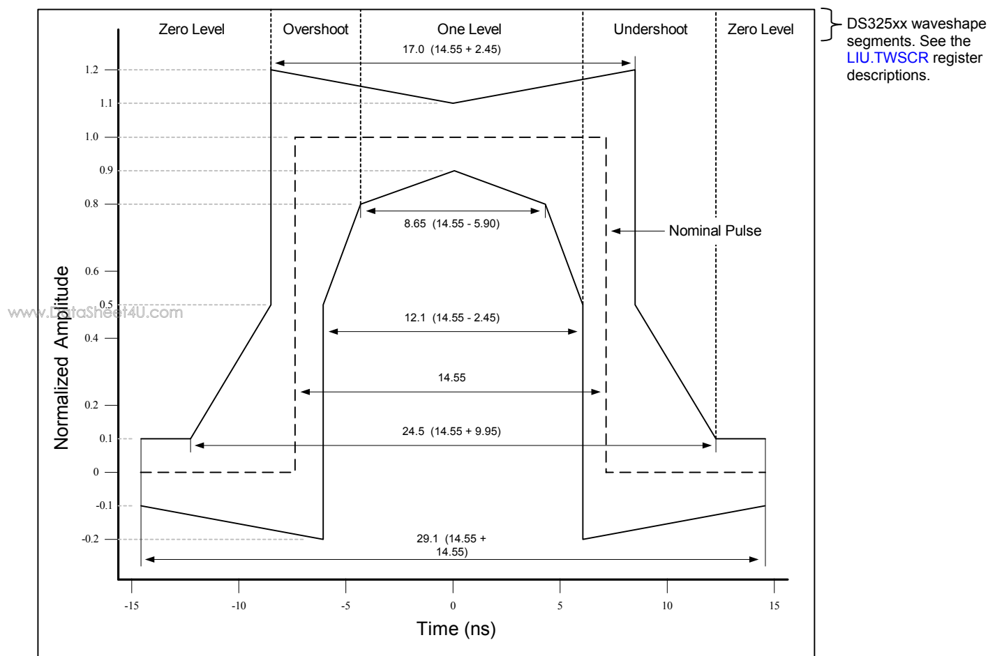
Figure 8-3. E3 Waveform Template
