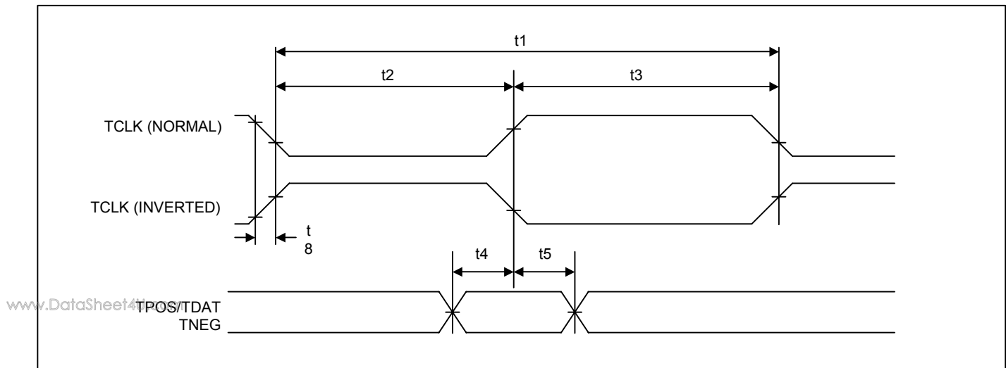
Figure 11-1. Transmitter Framer Interface Timing Diagram
