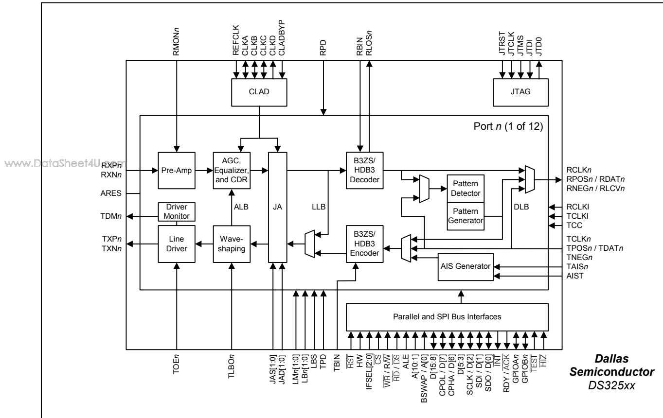
Figure 2-1. Block Diagram
