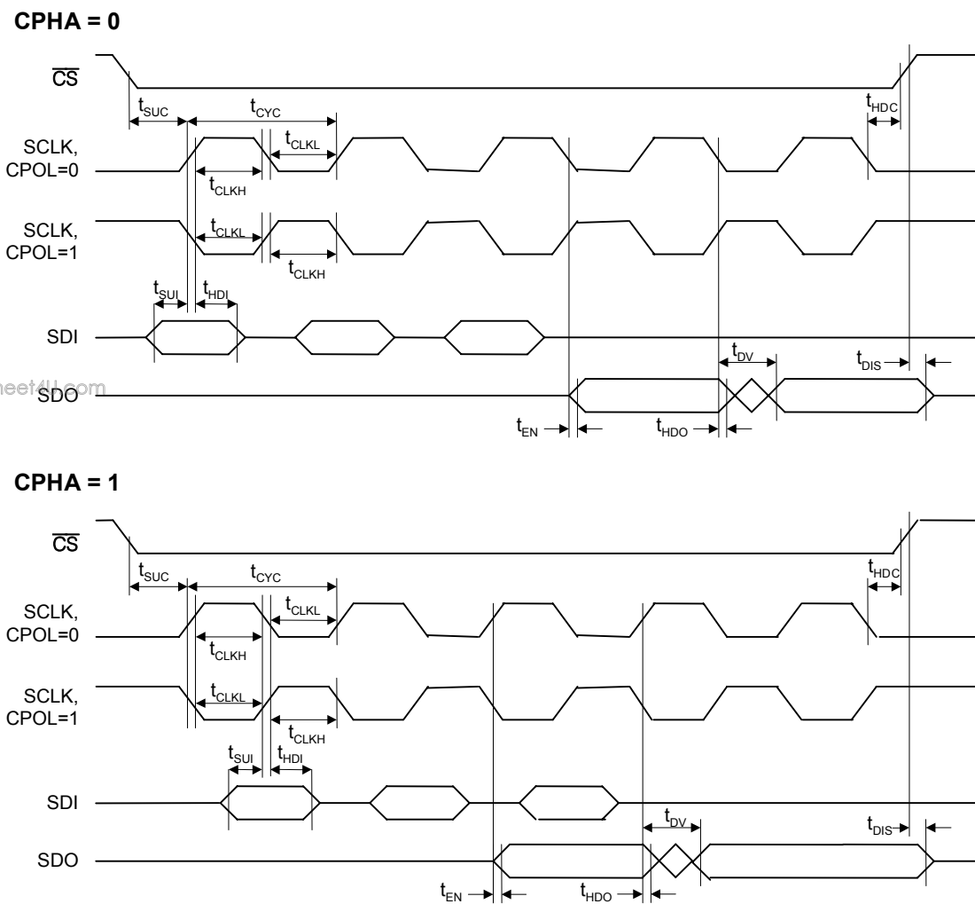
Figure 11-11. SPI Interface Timing Diagram
