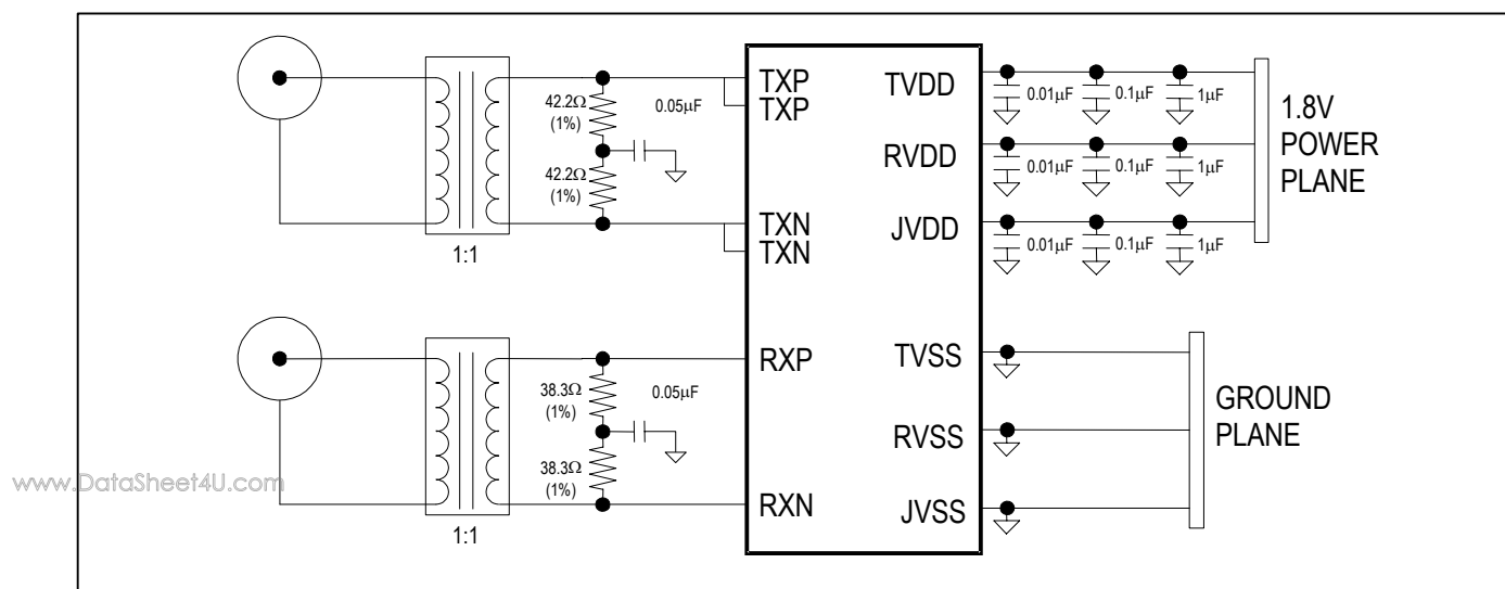
Figure 4-2. External Connections, Internal Termination Disabled
