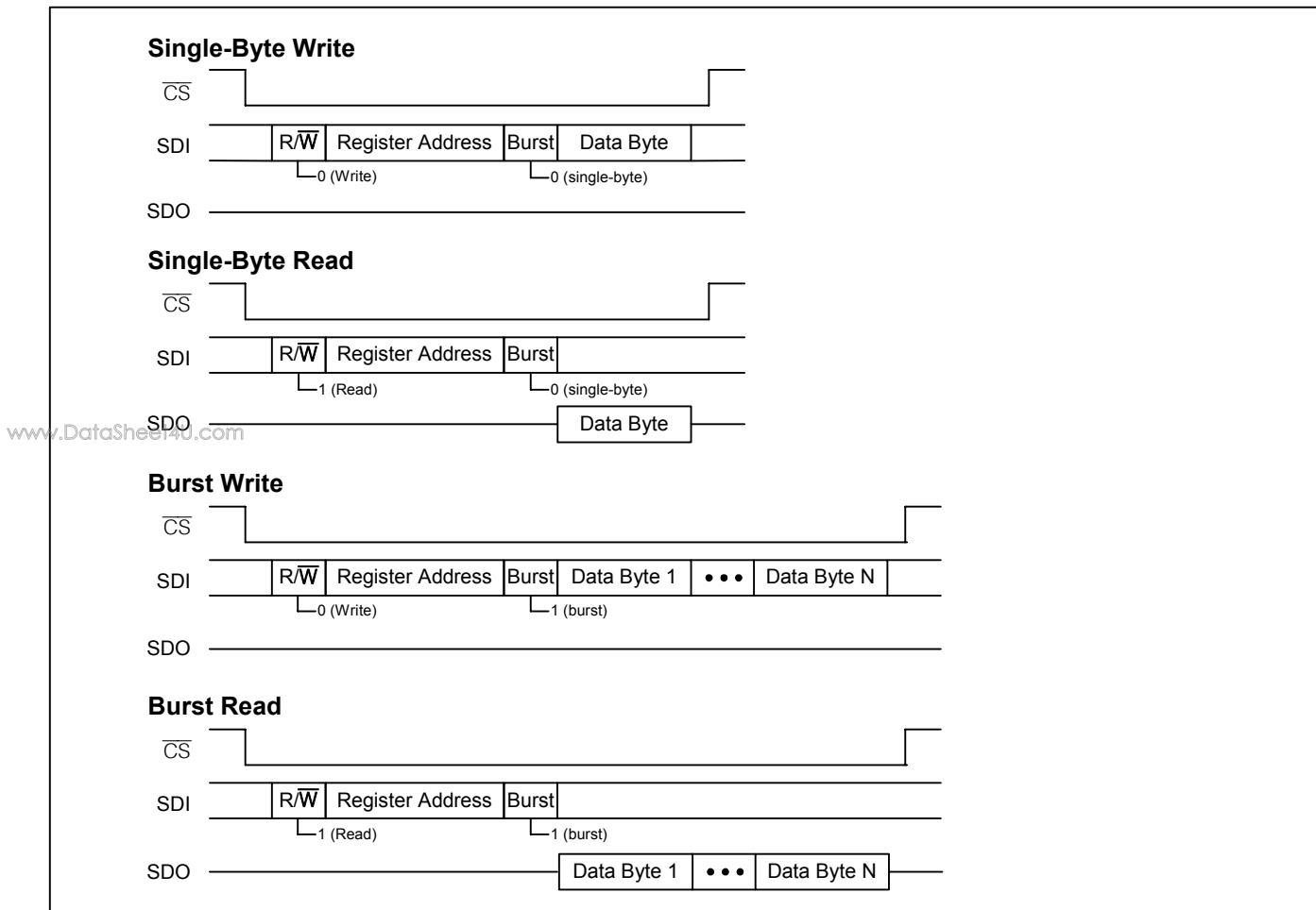
Figure 8-11. SPI Bus Transactions
