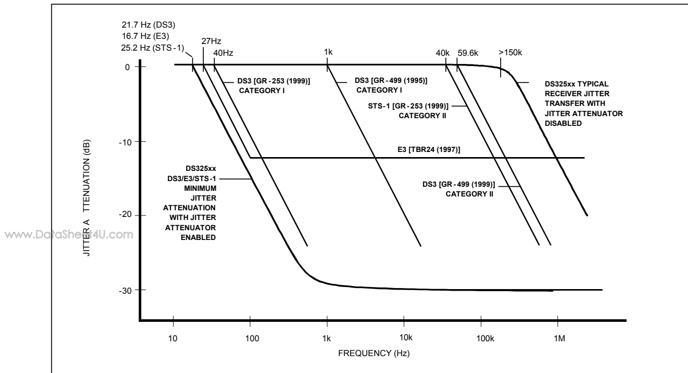
Figure 8-7. Jitter Attenuation/Jitter Transfer
