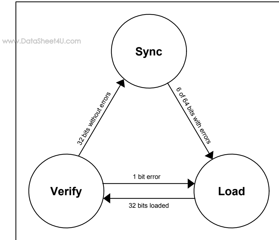
Figure 8-8. PRBS Synchronization State Diagram
