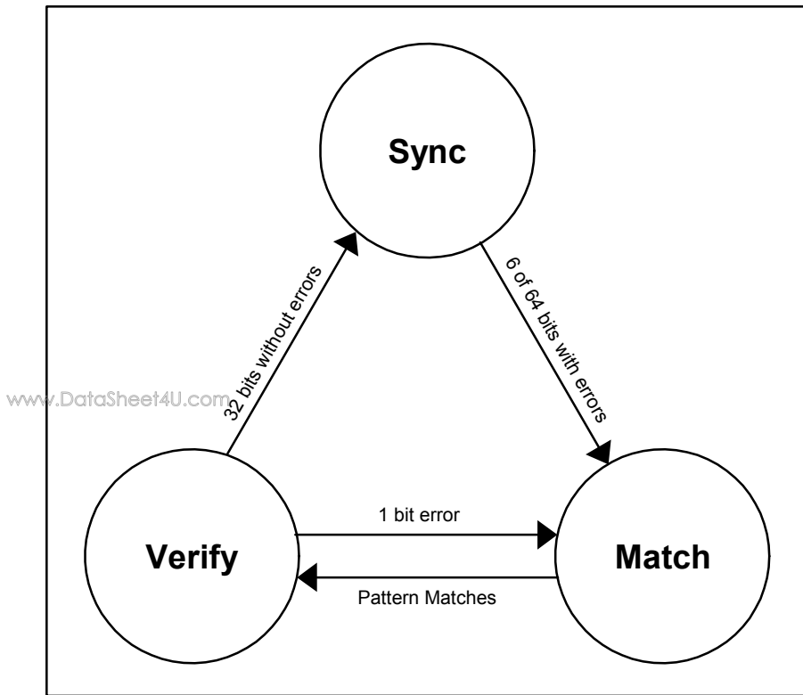
Figure 8-9. Repetitive Pattern Synchronization State Diagram
