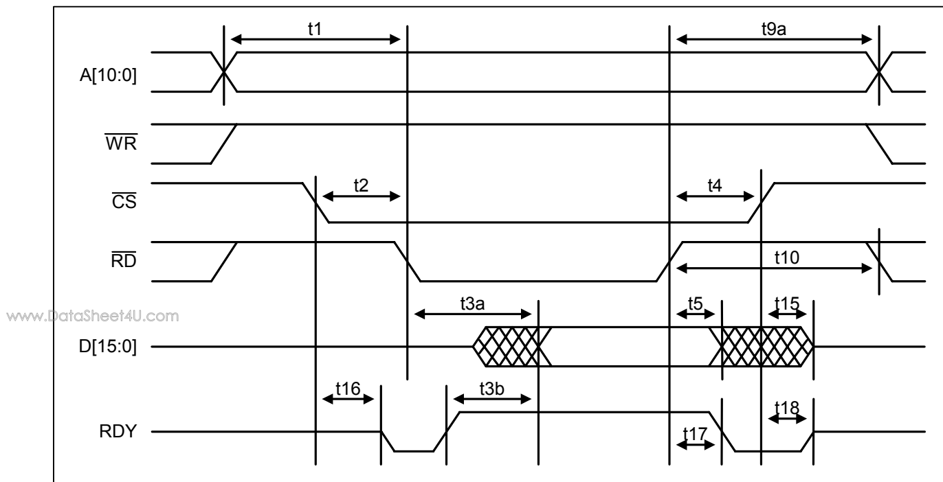
Figure 11-3. Parallel CPU Interface Intel Read Timing Diagram (Nonmultiplexed)
