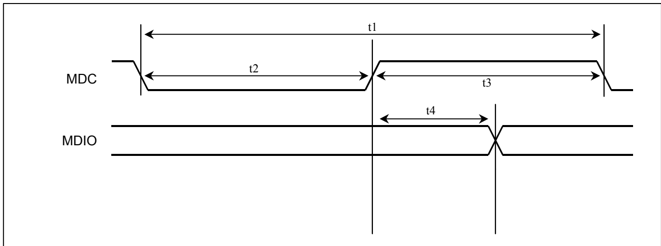
Figure 11-5. MDIO Timing
