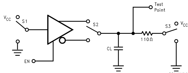
FIGURE 4. Driver Single-Ended TRI-STATE Test Circuit
