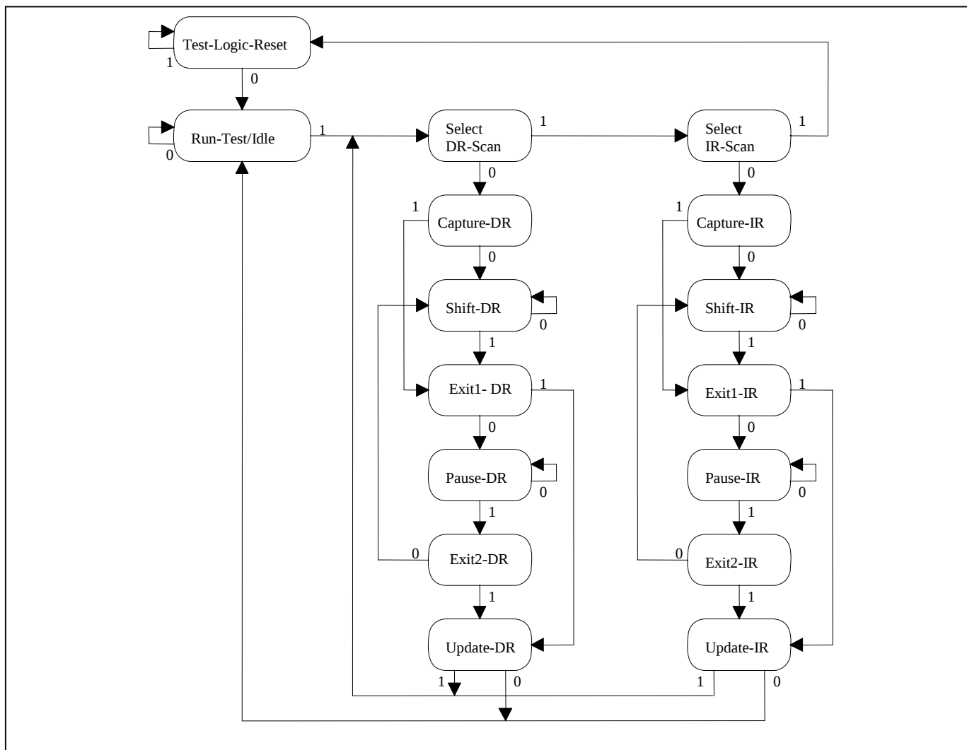
Figure 11-2. JTAG TAP Controller State Machine
