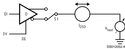
FIGURE 4. Driver I_{OSD}
