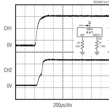
STARTUP DELAY ( V_{\text{MIRIN}} = 5\text{V} , I_{\text{MIROUT}} = 2.5\text{mA} )
