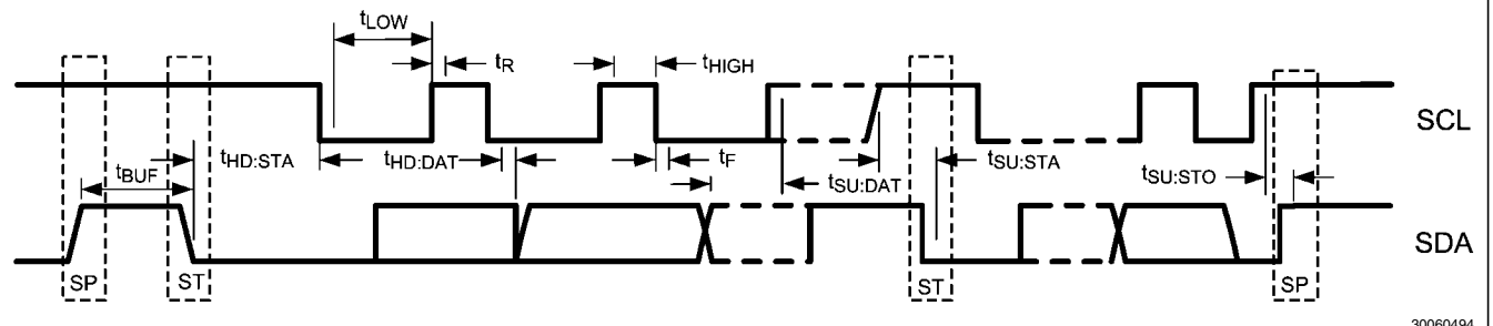
FIGURE 7. SMBus Timing Parameters
