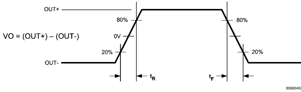
FIGURE 3. CML Output Transition Times
