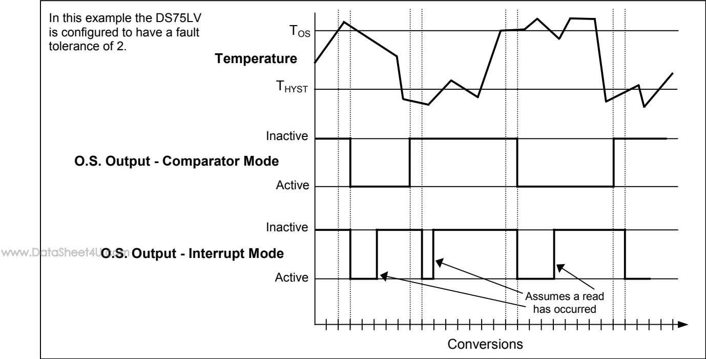
Figure 4. O.S. OUTPUT Operation Example
