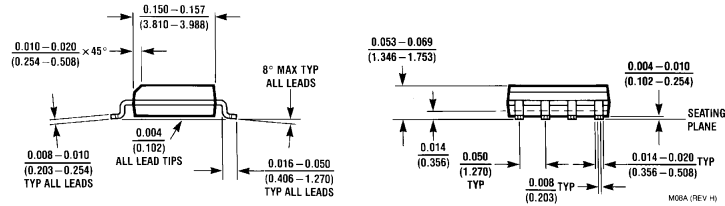
Molded Dual-In-Line Package (M) Order Number DS8614M-4, DS8615M-4, DS8616M-4 or DS8617M-4 NS Package Number M08A
