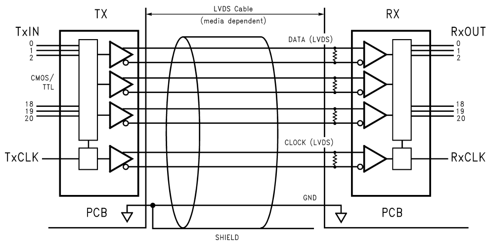
DS90CR218A
