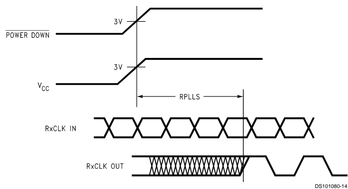
FIGURE 11. DS90CR218A (Receiver) Phase Lock Loop Set Time
