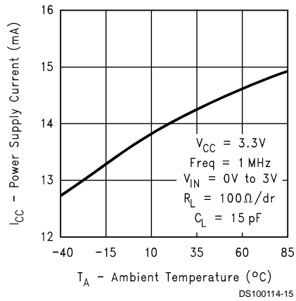
Power Supply Current vs Ambient Temperature
