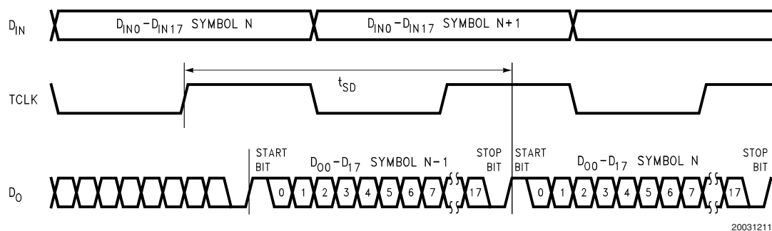
FIGURE 10. Serializer Delay
