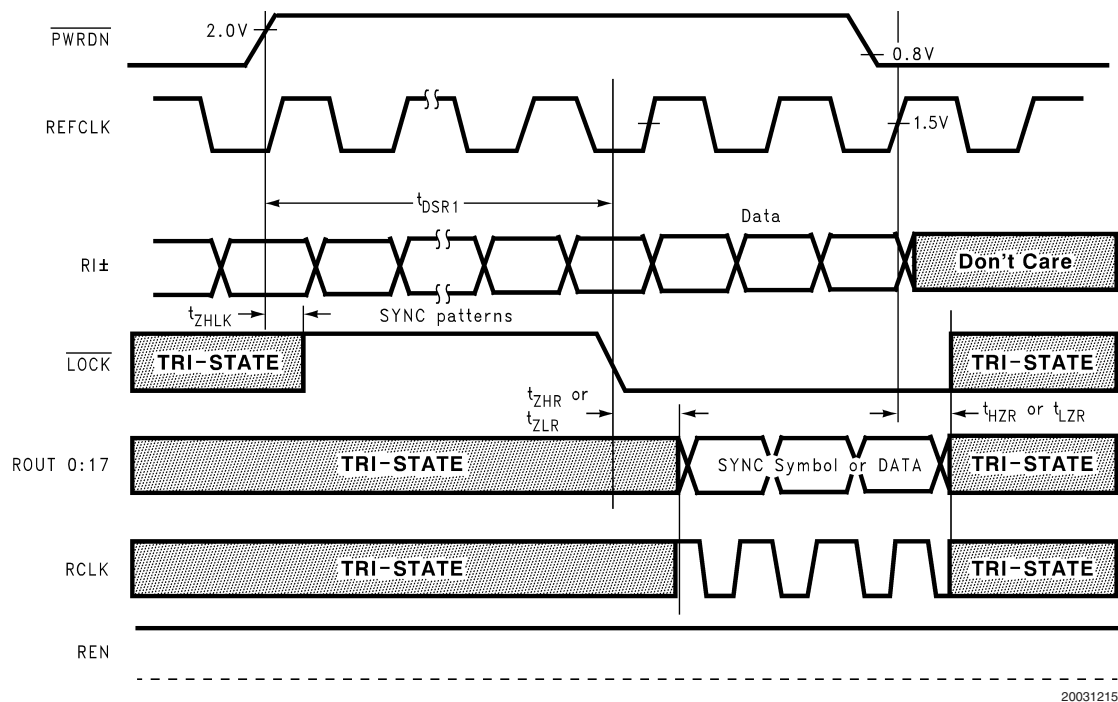
FIGURE 14. Deserializer PLL Lock Times and \overline{\text{PWRDN}} TRI-STATE Delays
