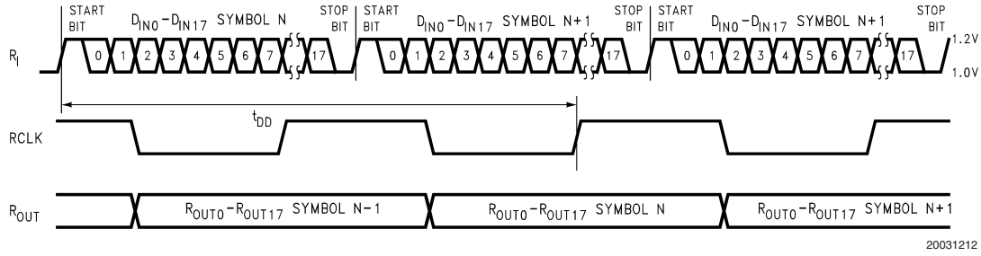
FIGURE 11. Deserializer Delay
