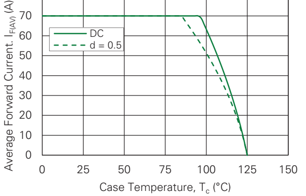
Figure 4. Average Forward Current vs. Case Temperature
