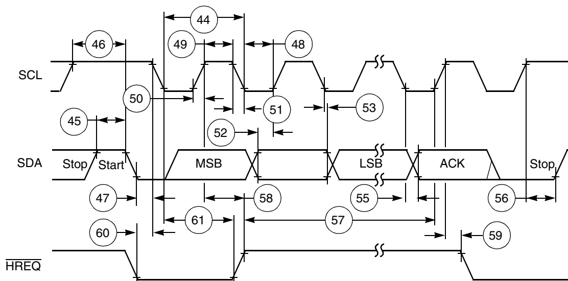
Figure 11. I²C Timing
