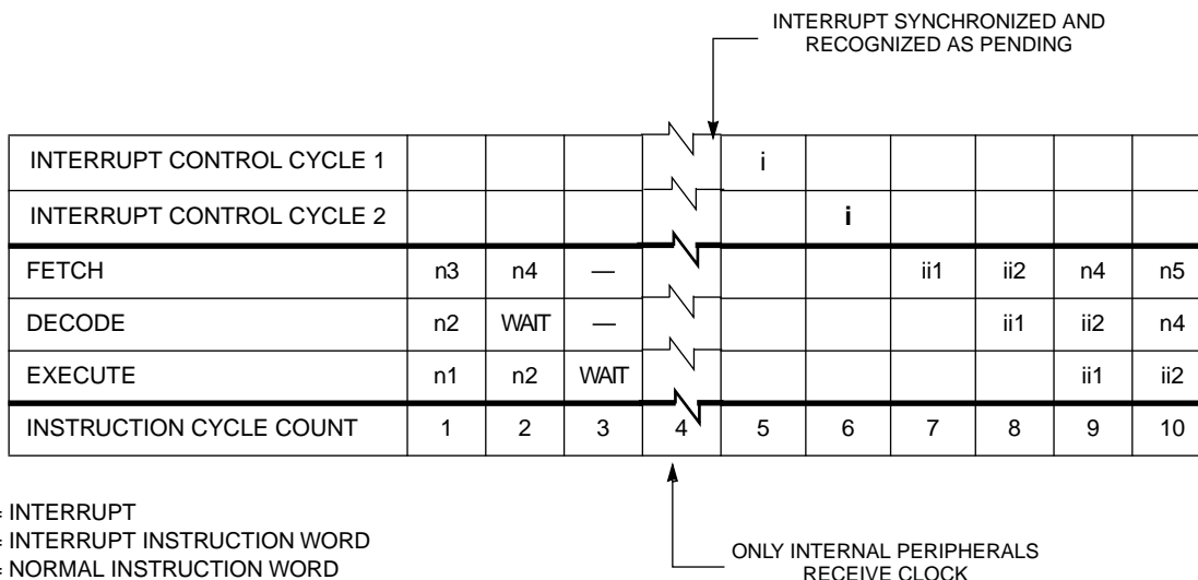
Figure 7-15 Wait Instruction Timing
