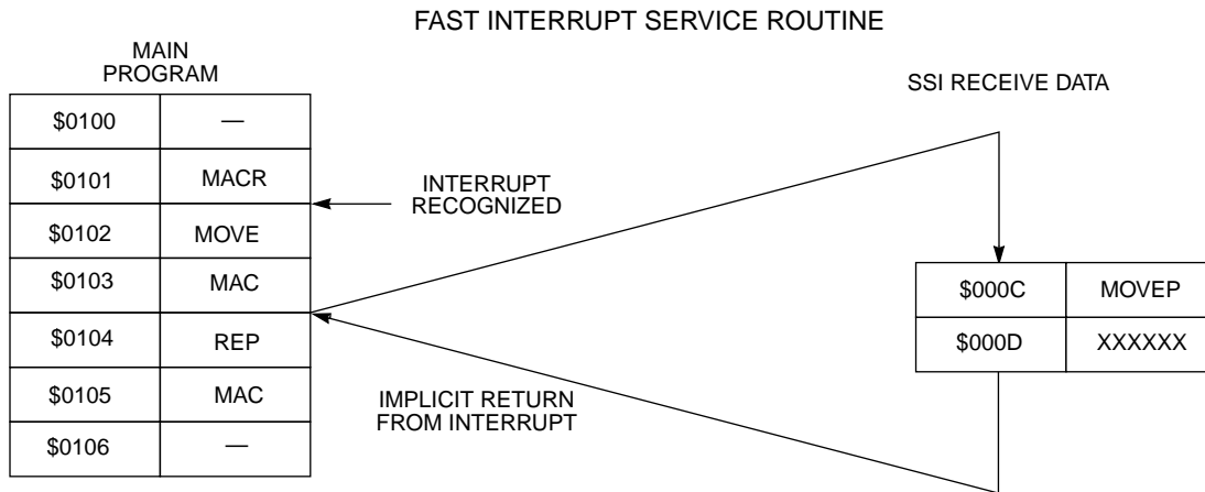
(a) DSP56K Fast Interrupt
