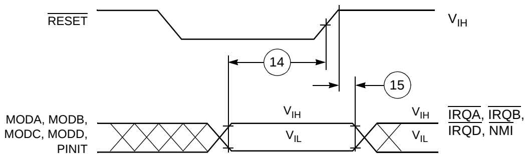
Figure 5. Reset Timing
