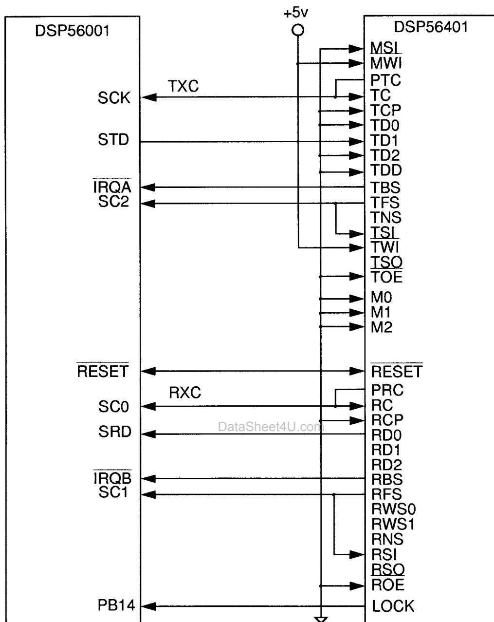
Figure 7-2 DSP56001 Asynchronous Transmit/Receive Interface
