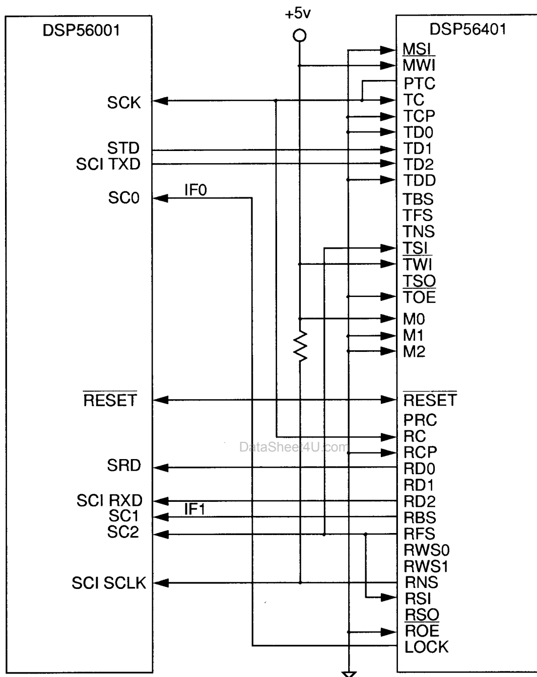
Figure 7-3 DSP56001 Synchronous Transmit/Receive Interface
