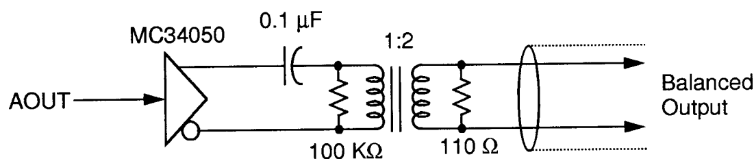
Figure 8-2 Balanced AES/EBU and CP340 Transmitter
