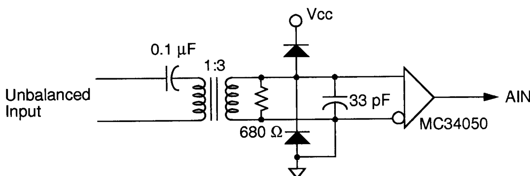
Figure 8-3 Unbalanced CP340 Receiver
