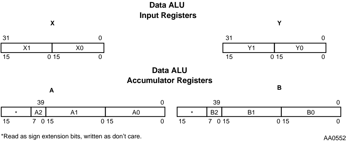
Figure 3-8 DSP56600 Core Programming Model
