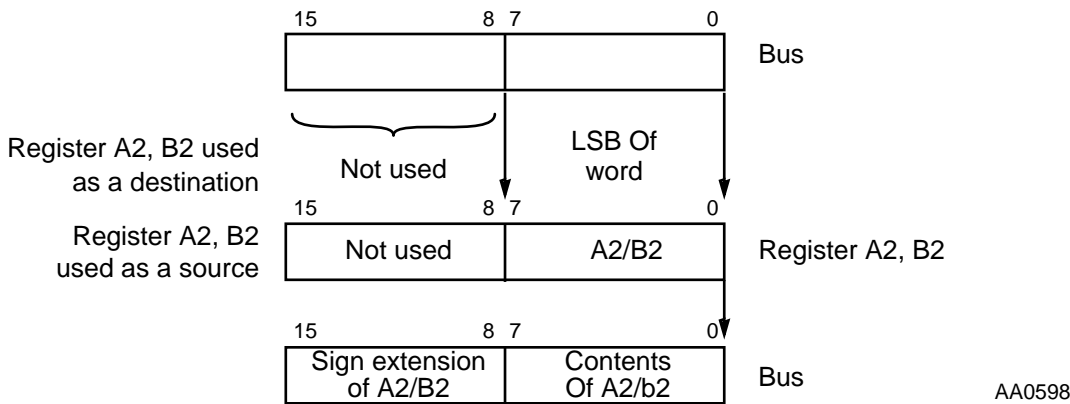
Figure A-3 Reading and Writing the ALU Extension Registers
