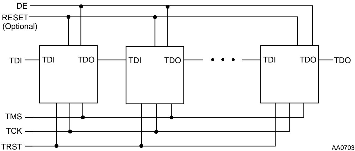
Figure 10-7 OnCE Multiprocessor Configuration
