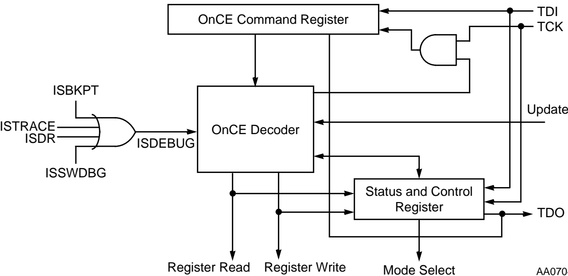
Figure 10-8 OnCE Controller
