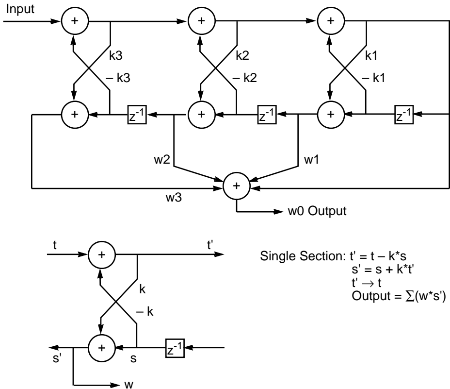
Figure C-4 General Lattice Filter
