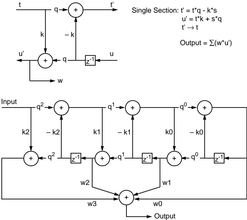
Figure C-5 Normalized Lattice Filter
