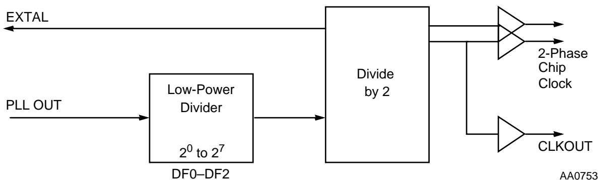
Figure 8-5 CLKGEN Block Diagram
