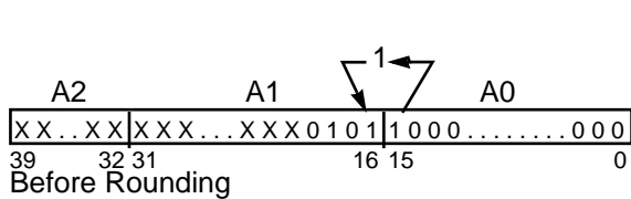
Figure 3-4 Convergent Rounding (No Scaling)
