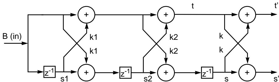
Figure C-2 FIR Lattice Filter
