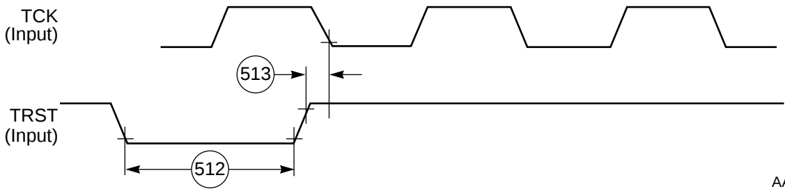
Figure 2-28 \overline{\text{TRST}} Timing Diagram
