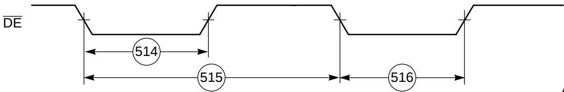
Figure 2-29 OnCE—Debug Request
