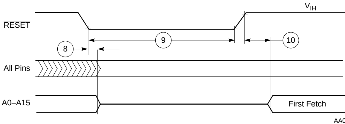
Figure 2-3 Reset Timing
