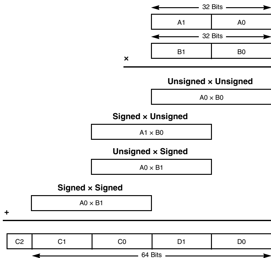
Figure 5-24. 32-Bit × 32-Bit → 64-Bit Signed Integer Multiplication
