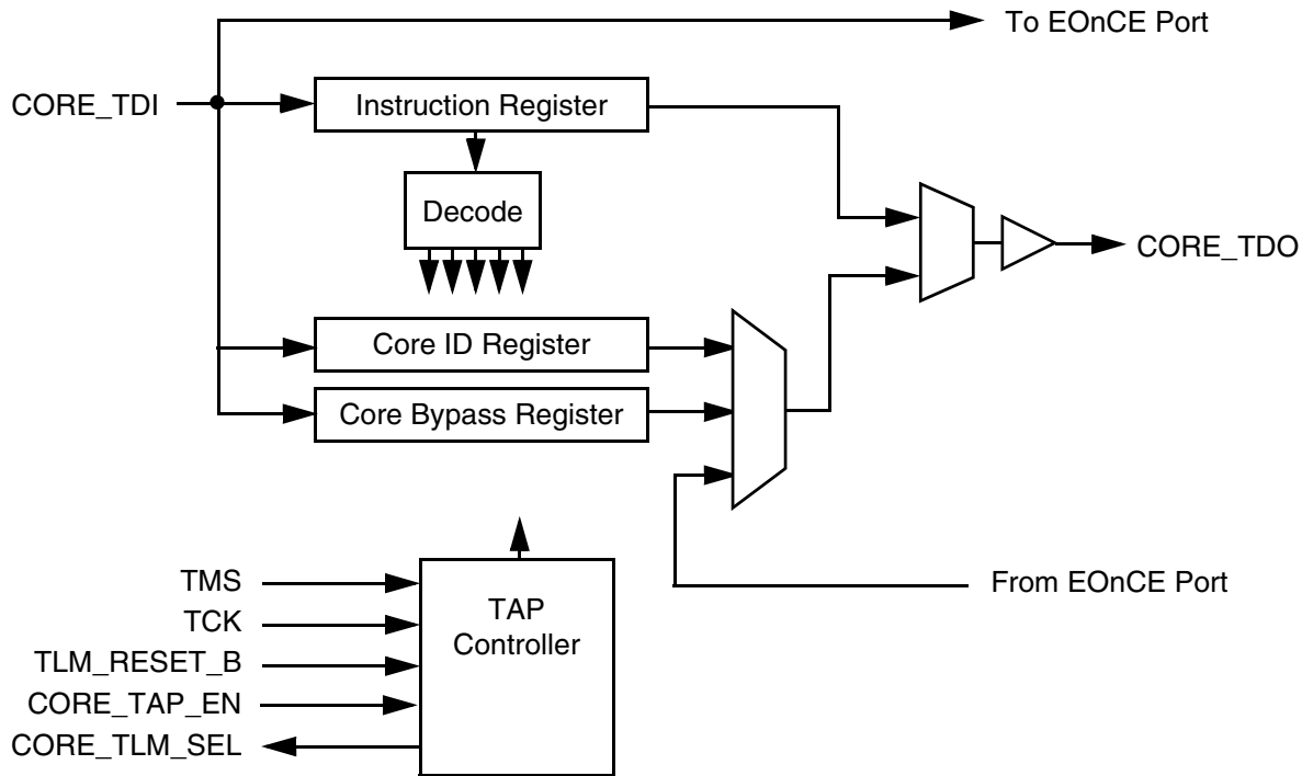
Figure 11-16. Core JTAG Block Diagram
