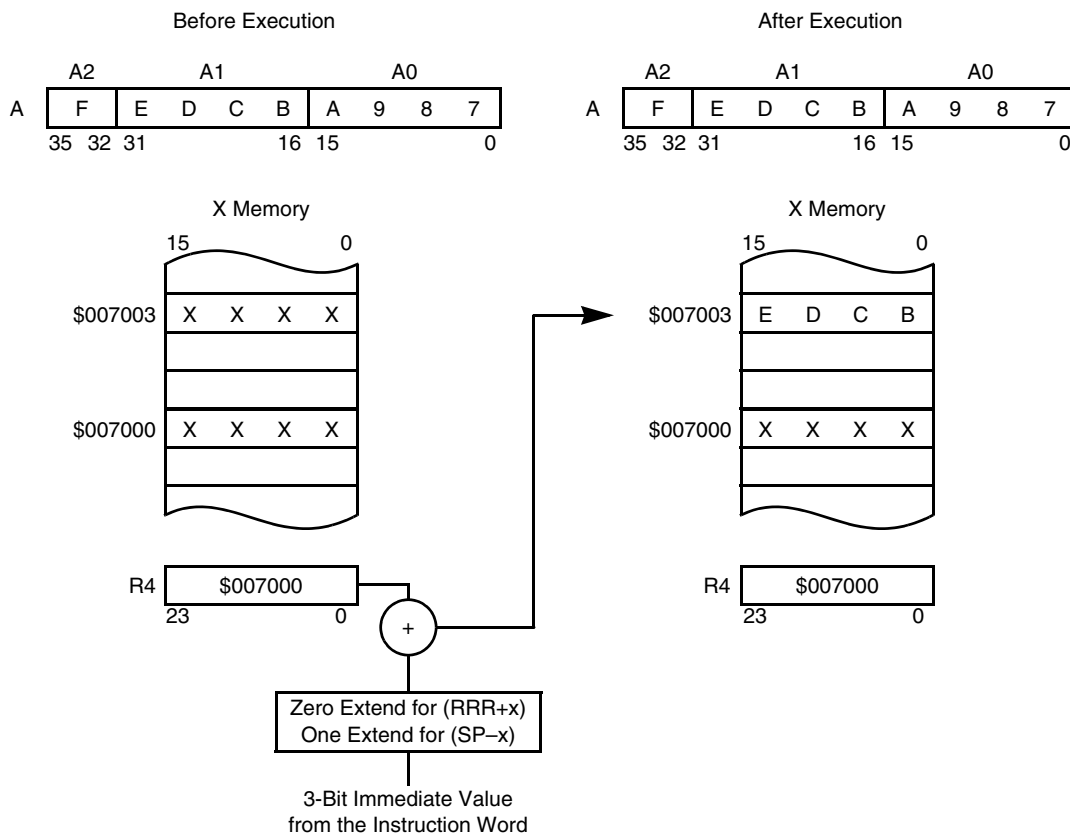
Indexed by 3-Bit Displacement Example: MOVE.W A1, X: (R4+3)
