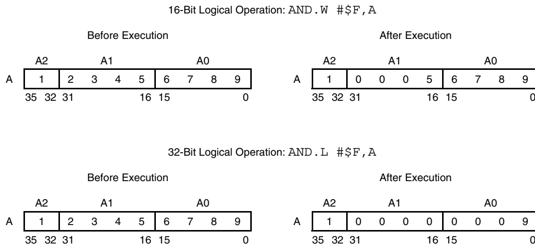
Figure 5-17. 16- and 32-Bit Logical Operations
