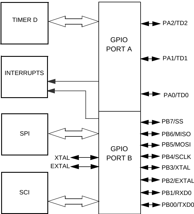
Figure 7-1. Block Diagram Showing 56F801 GPIO Connections
