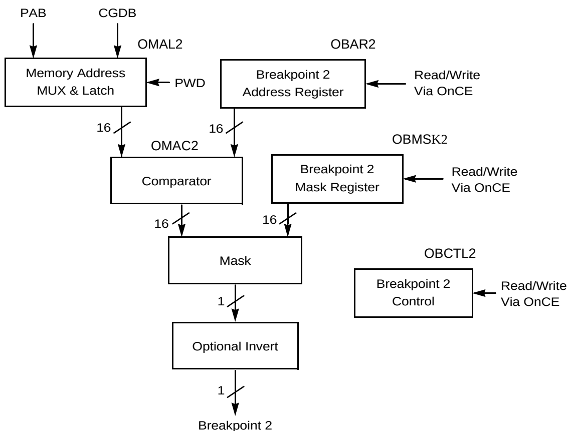
Figure 17-22. Breakpoint 2 Unit
