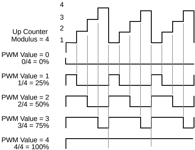
Figure 11-7. Edge-Aligned PWM Pulse Width
