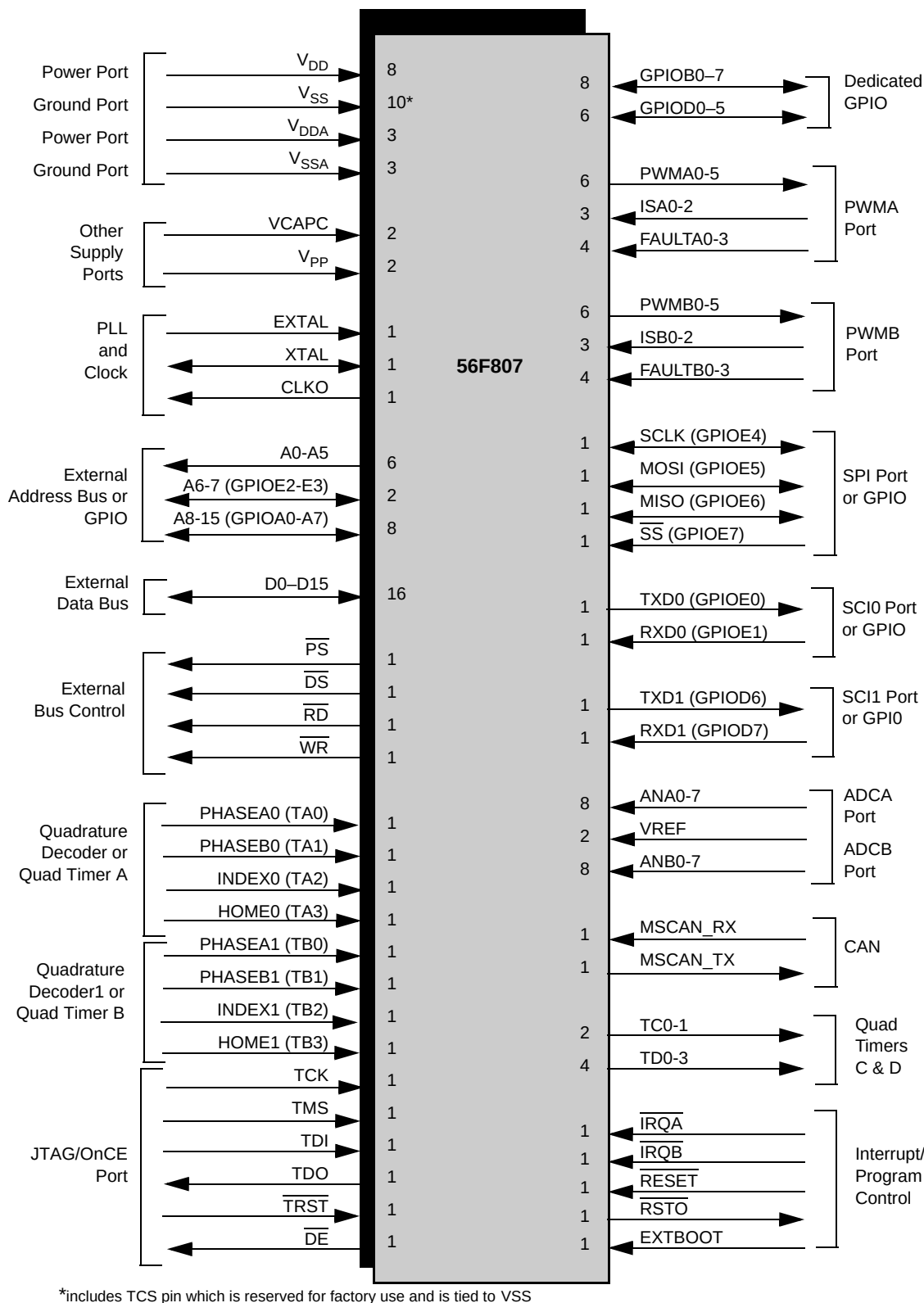
Figure 2-5. 56F807 Signals Identified by Functional Group 1
