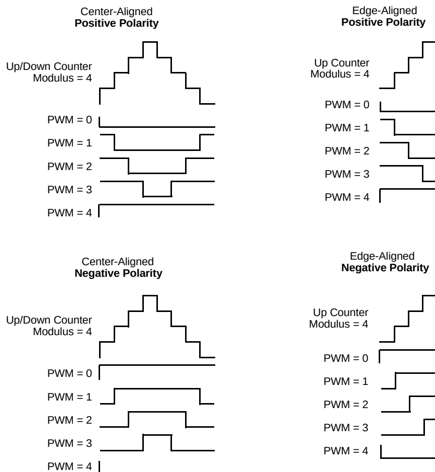
Figure 11-19. PWM Polarity
