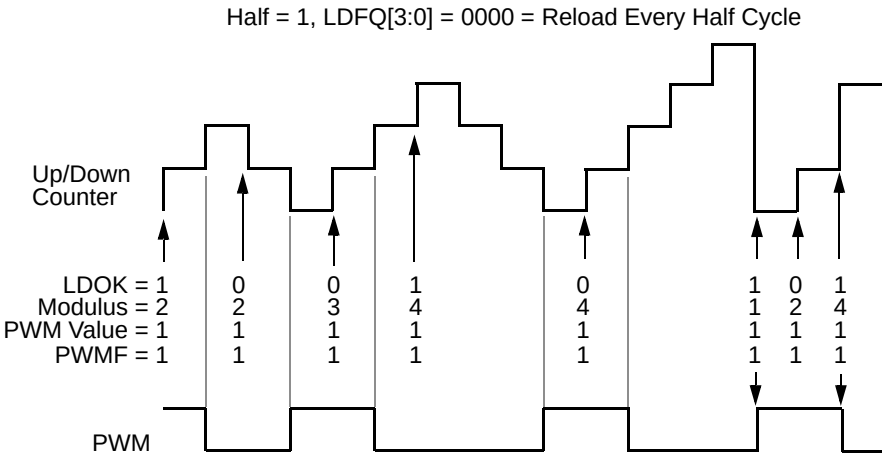
Figure 11-26. Half Cycle Center-Aligned Modulus Loading
