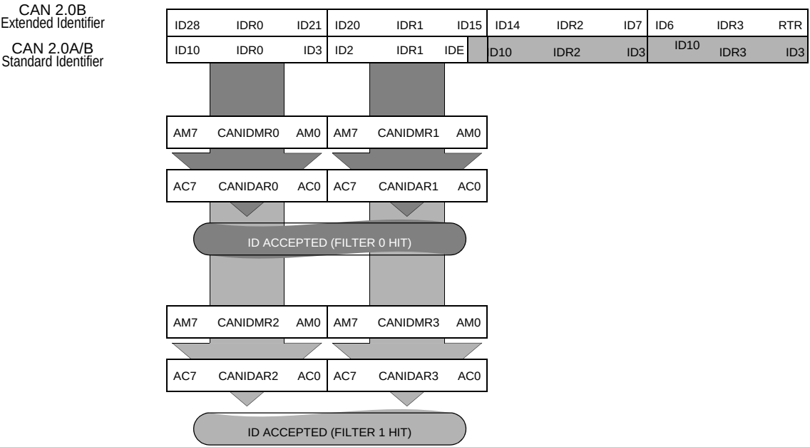
Figure 8-4. 16-Bit Maskable Identifier Acceptance Filters
