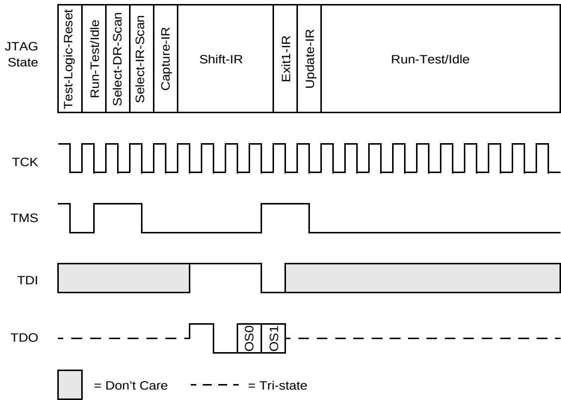
Figure 17-26. Loading DEBUG_REQUEST
