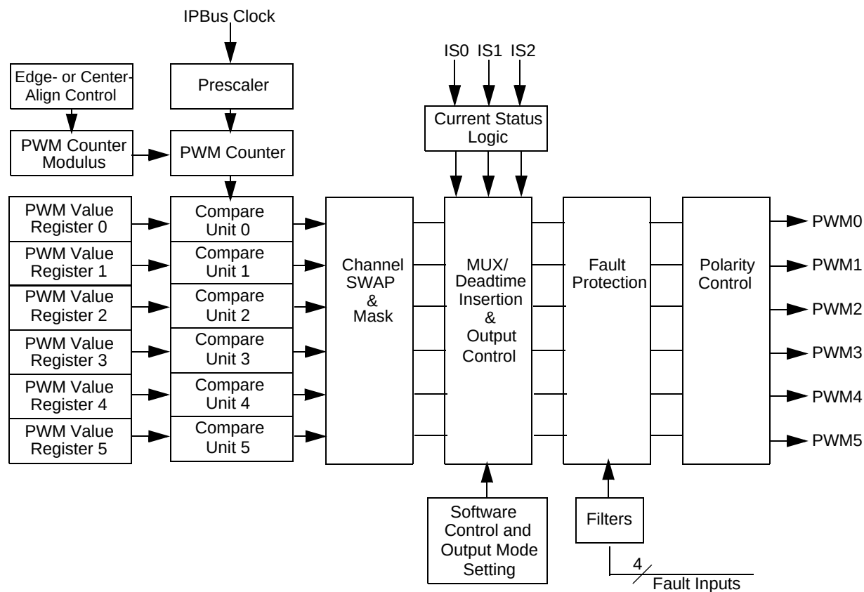
Figure 11-1. PWM Block Diagram
