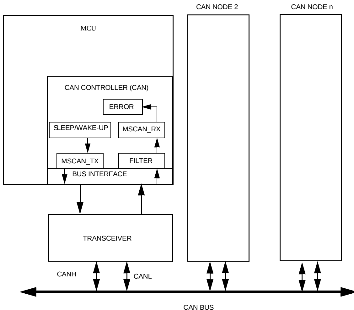
Figure 8-8. CAN System
