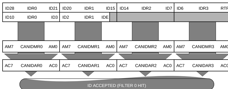
Figure 8-3. 32-Bit Mask Identifier Acceptance Filter
