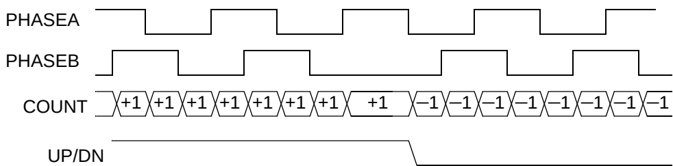
Figure 14-2. Timing Diagram
