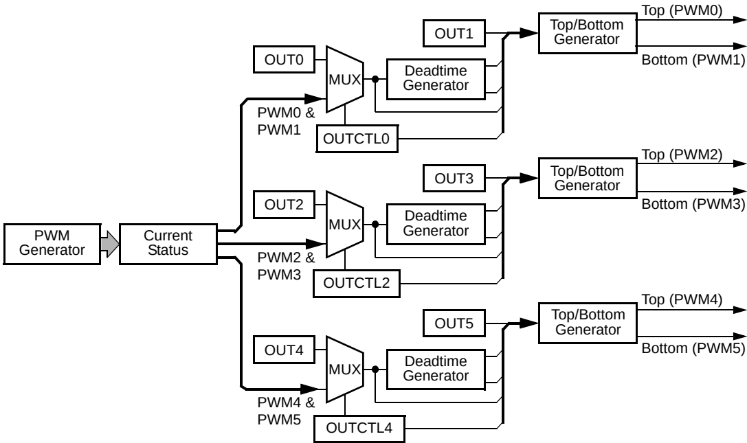
Figure 11-10. Deadtime Generators
