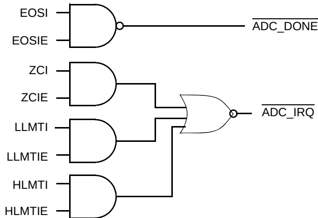
Figure 9-14. ADC Interrupt
