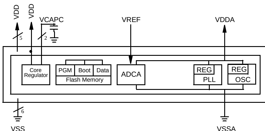
Figure 2-8. 56F803 Power and Ground Pins
