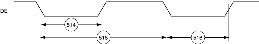
Figure 2-44. OnCE—Debug Request
