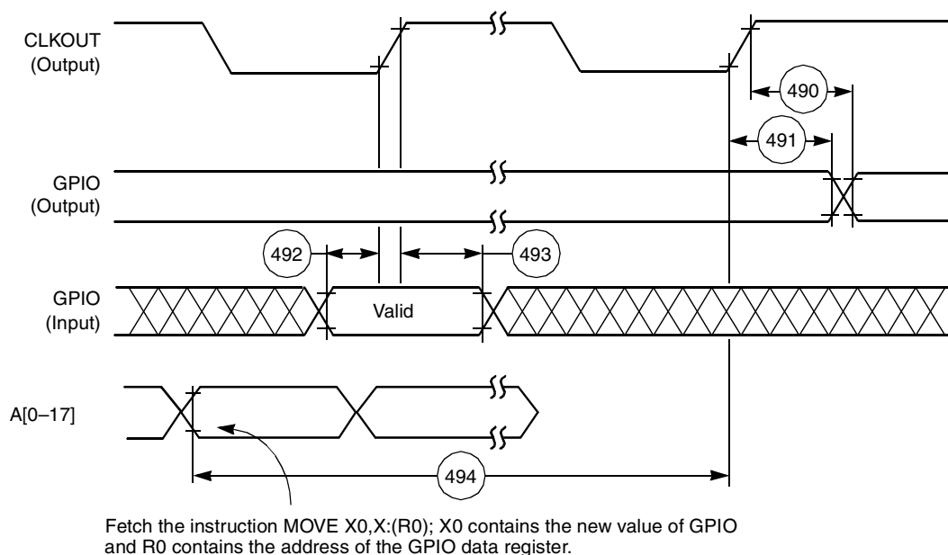
Figure 2-39. GPIO Timing
