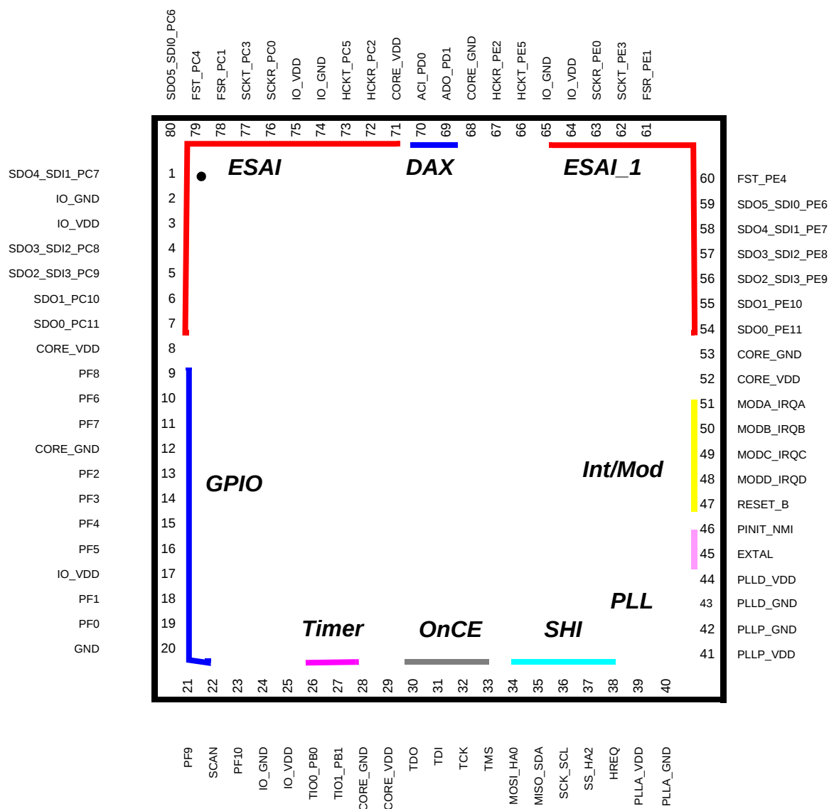
Figure 24. DSP56371 Pinout
