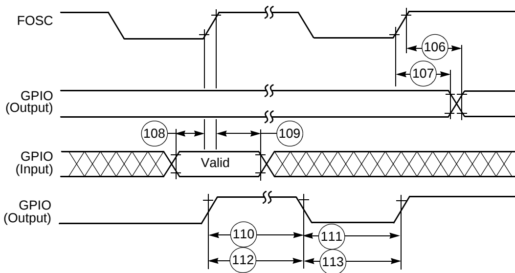
Figure 20. GPIO Timing
