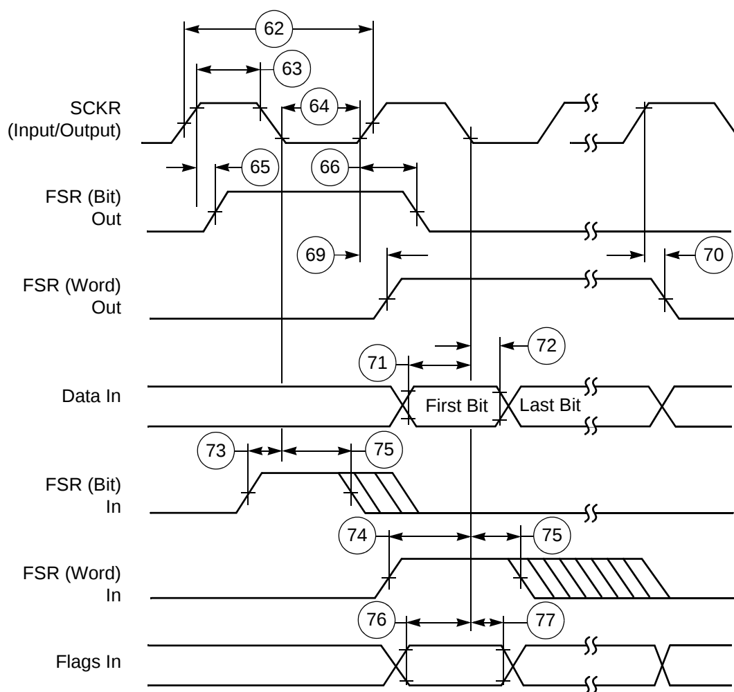
Figure 15. ESAI Receiver Timing
