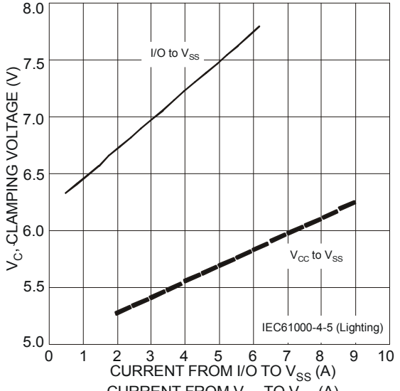
Figure 3 Clamping Voltage Characteristics
