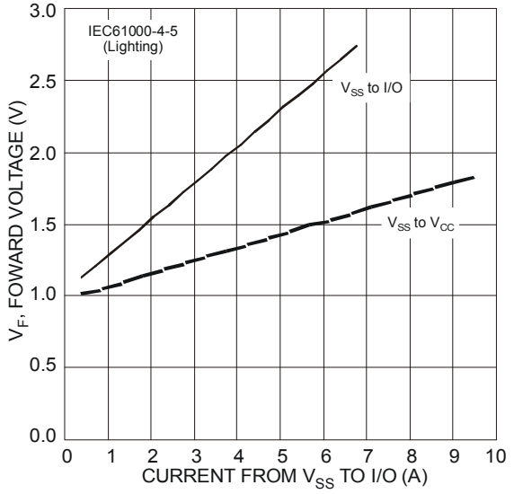
Figure 4 Forward Voltage Characteristics
