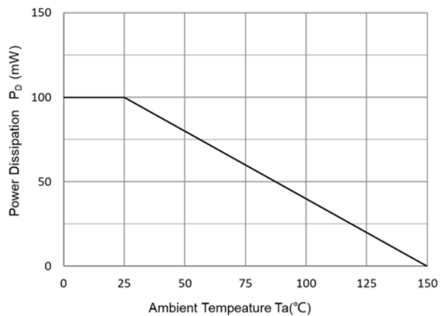
Fig 5: PD-Ta Curve
