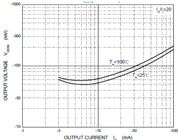
Fig 4: Output Voltage Characteristics
