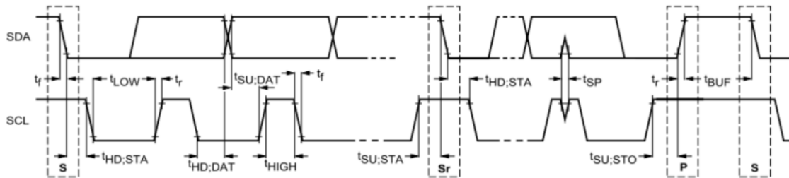
I 2 C interface
