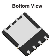
DFN5X6-8L Pin Configuration
