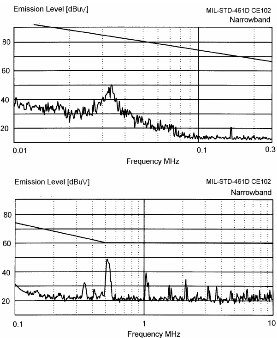
Figure 10 – MIL-STD-461D DVETR2800D
