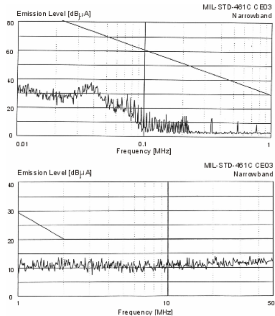
Figure 9 – MIL-STD-461C DVETR2800D
