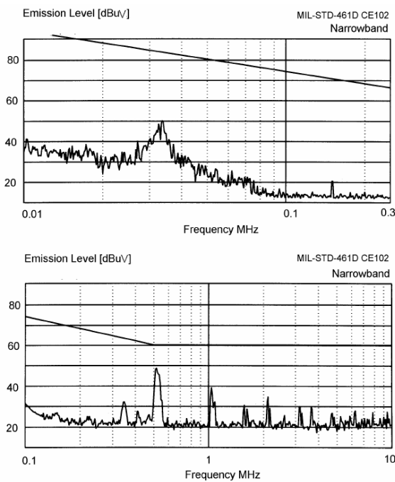
Figure 12 – MIL-STD-461D DVETR2800S
