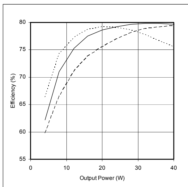
Figure 10 – DVETR2815S Efficiency (%) vs. Output Power (W)
