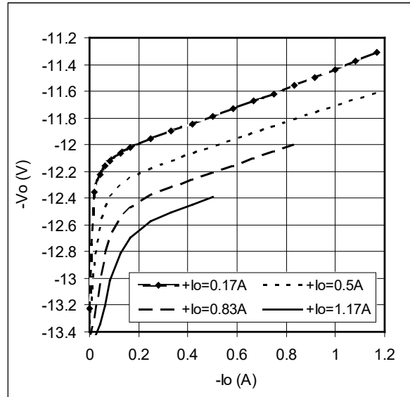
Figure 11 – DVHF2812D
