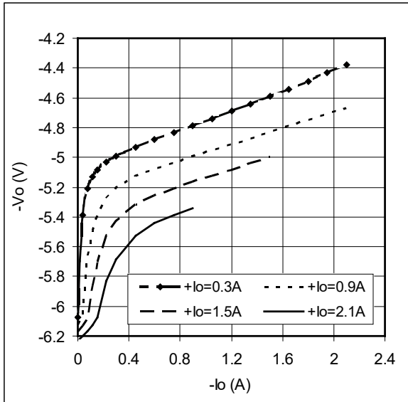
Figure 10 – DVHF2805D
