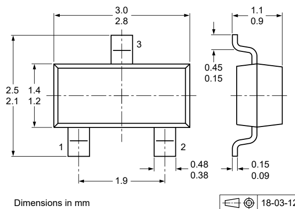
Fig. 8. Package outline SOT23
