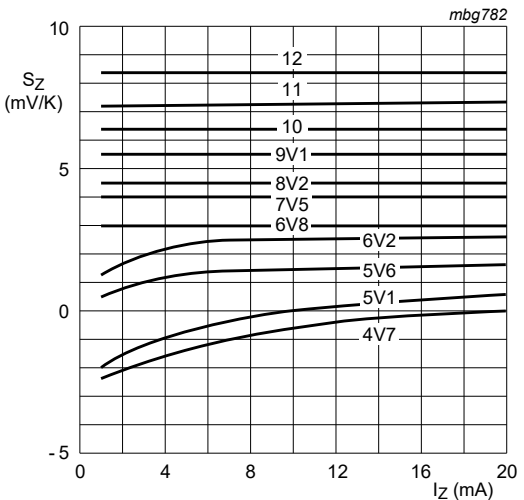
Fig. 4. Per diode: Temperature coefficient as a function of working current; typical values (DZ23-C4V7 to DZ23-C12)
