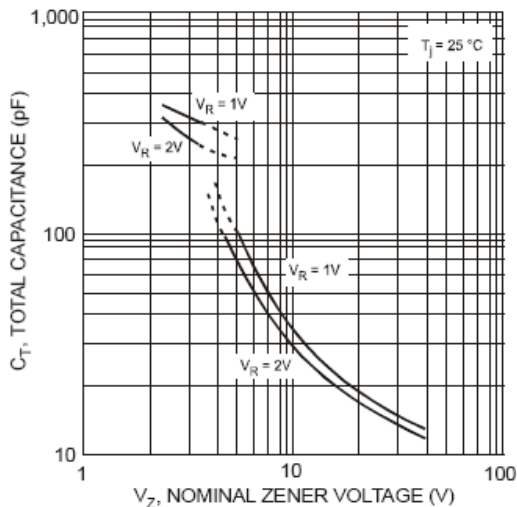
Fig. 5 Typical Total Capacitance vs. Nominal Zener Voltage
