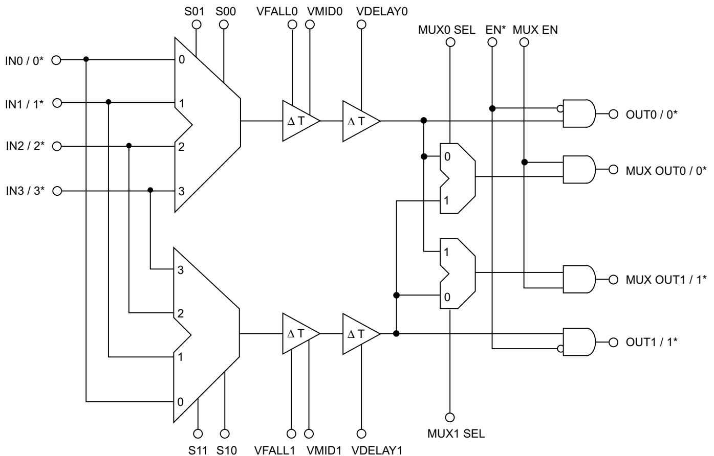
Figure 1. Edge142 Block Diagram
