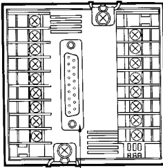
Communications connector (RS-232C and BCD connector is shown.)
