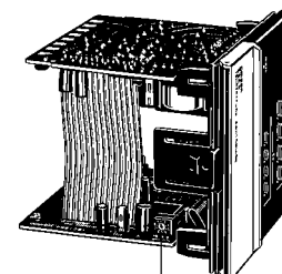
Temperature sensor selector (SW206, INPUT)
