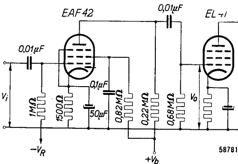
Fig. 5 Circuit diagram showing the EEF 42 as a resistance-coupled A.F. amplifier with control ( -V_R ) on the grid.
