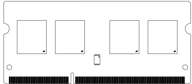
Figure 1: 204-Pin SODIMM (MO-268 R/C B4)
