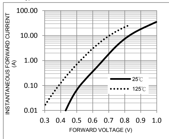
FIG. 2-Typical Forward Characteristics
