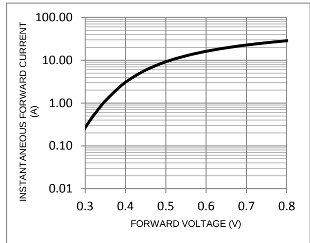
FIG. 2-Typical Forward Characteristics
