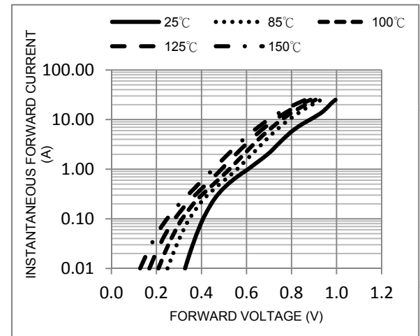
FIG. 2-Typical Forward Characteristics
