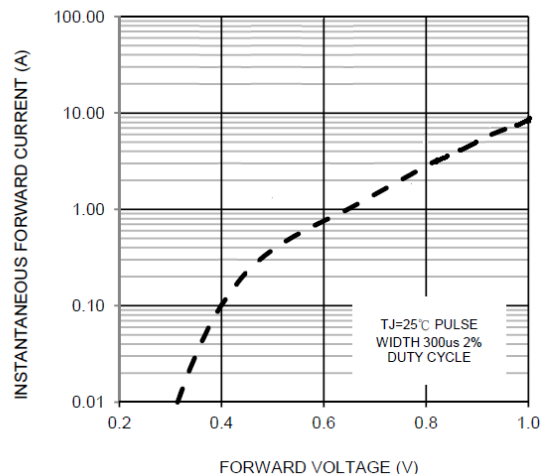
FIG. 2-TYPICAL FORWARD CHARACTERISTICS
