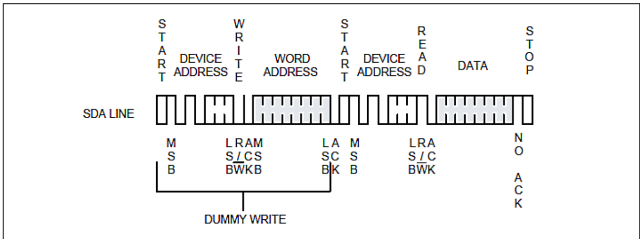
Figure 8: Random Read
