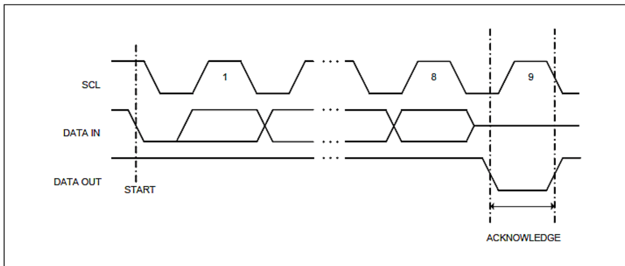
Figure 3: Output Acknowledge
