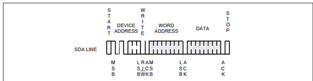
Figure 5: Byte Write
