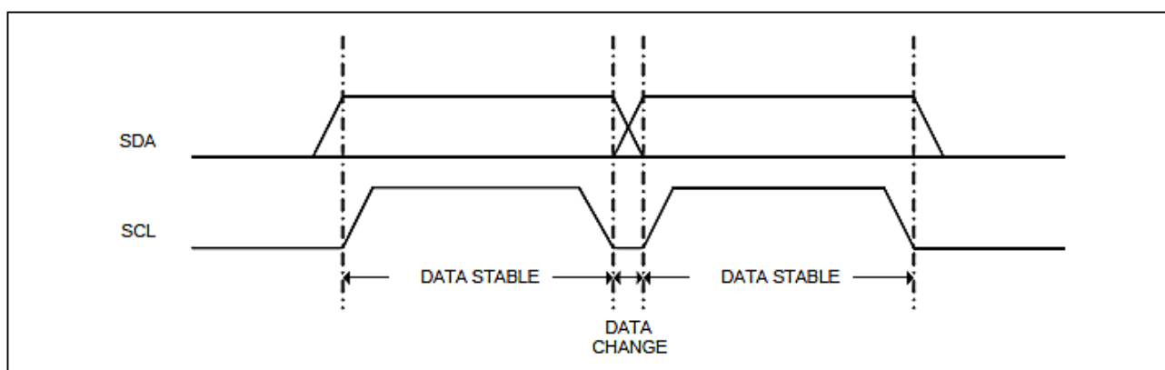
Figure 1: Data Validity
