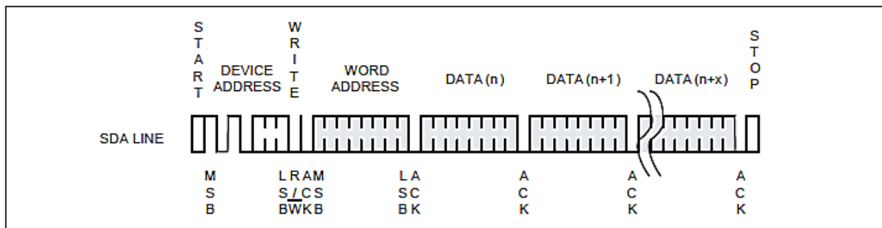
Figure 6: Page Write
