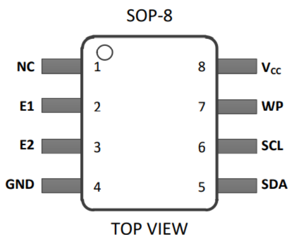
Figure 1–1 Pin Configuration
