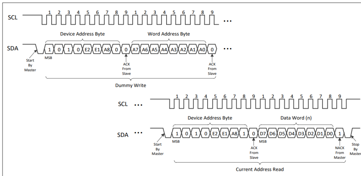
Figure 5–11 Random Read
