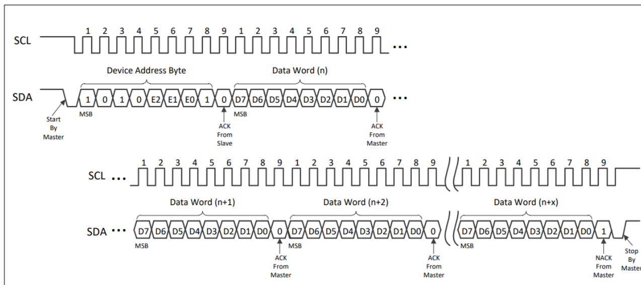
Figure 5–12 Sequential Read
