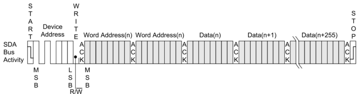
Figure 7. Page Write
