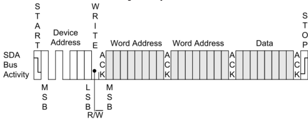
Figure 6. Byte Write
