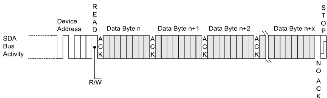
Figure 10. Sequential Read
