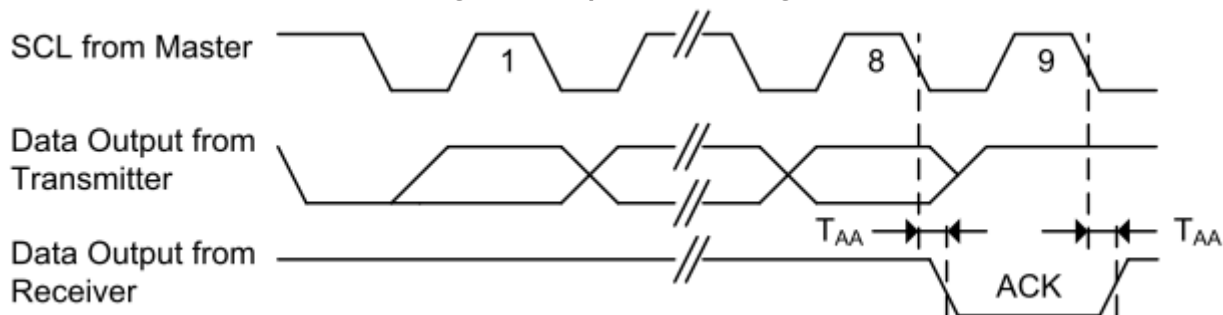
Figure 2. output Acknowledge
