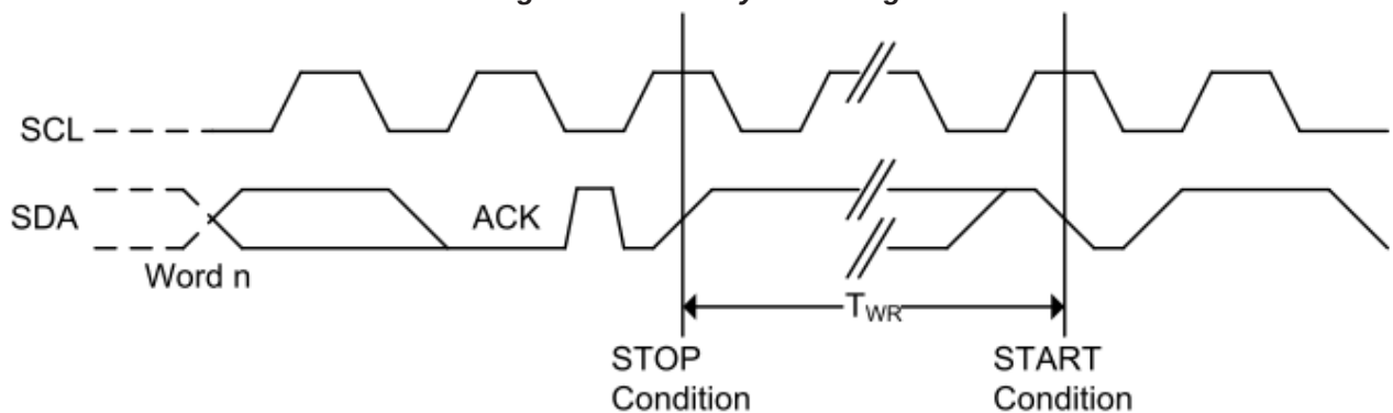
Figure 12. Write Cycle Timing
