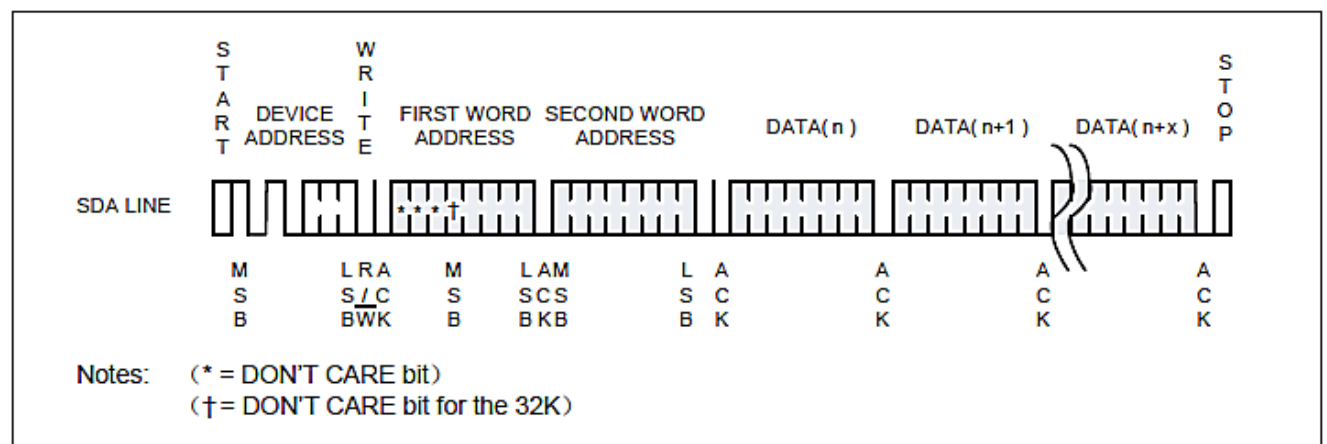
Figure 6: Page Write
