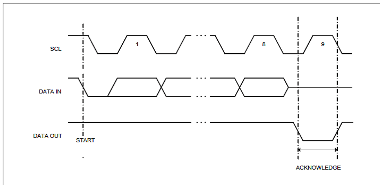
Figure 3: Output Acknowledge
