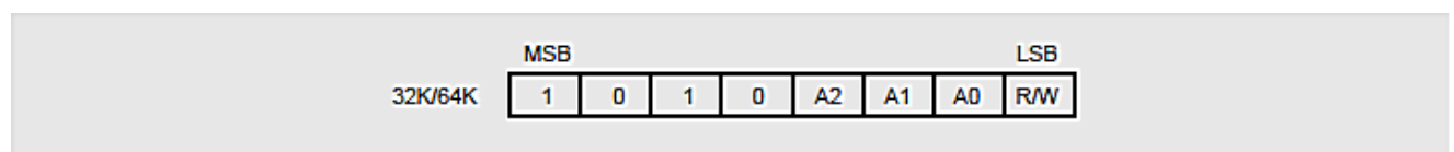
Figure 5: Byte Write
