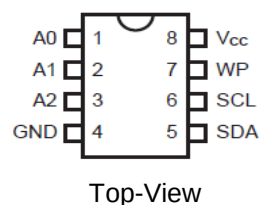
PDIP-8 (EC24C32A/64A)
