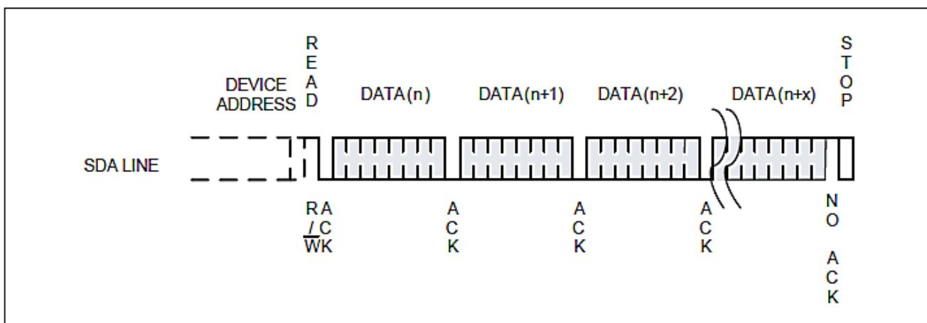
Figure 9: Sequential Read
