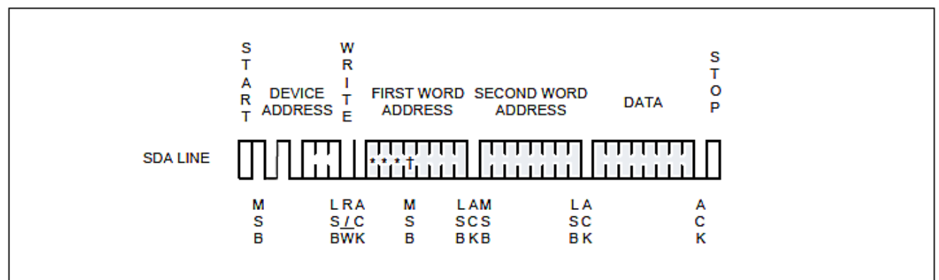
Figure 6: Page Write
