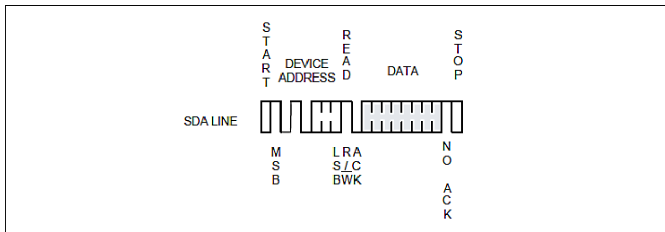
Figure 8: Random Read
