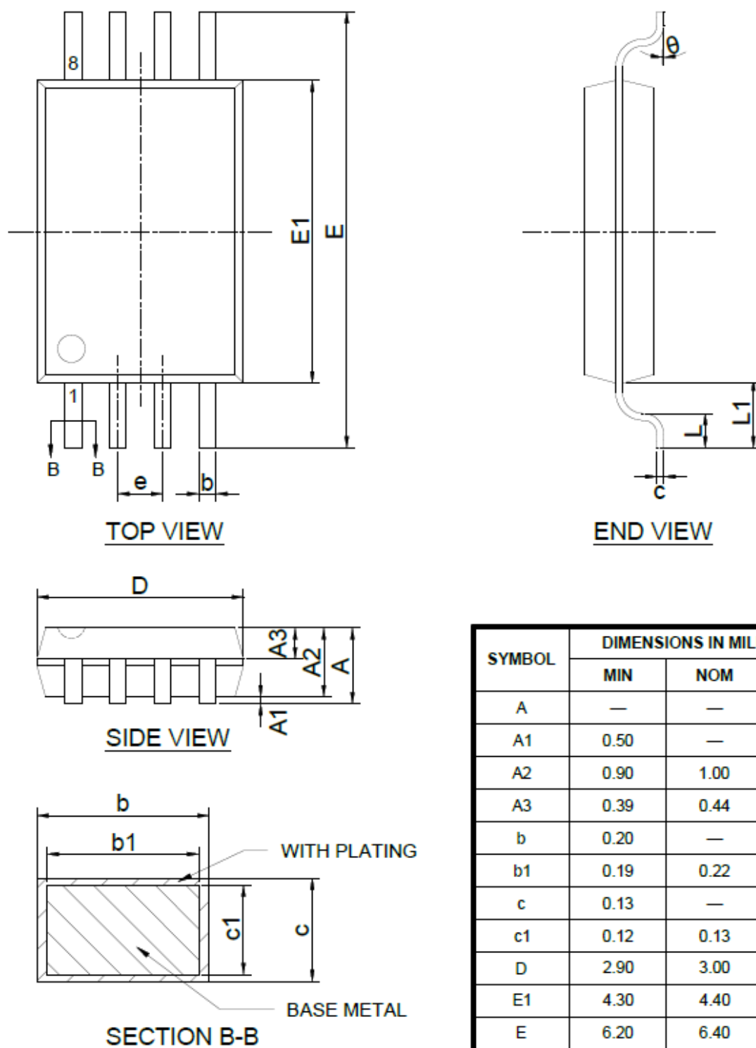
Figure 9–2 8-pad 3.0 x 4.4mm TSSOP Package Outline
