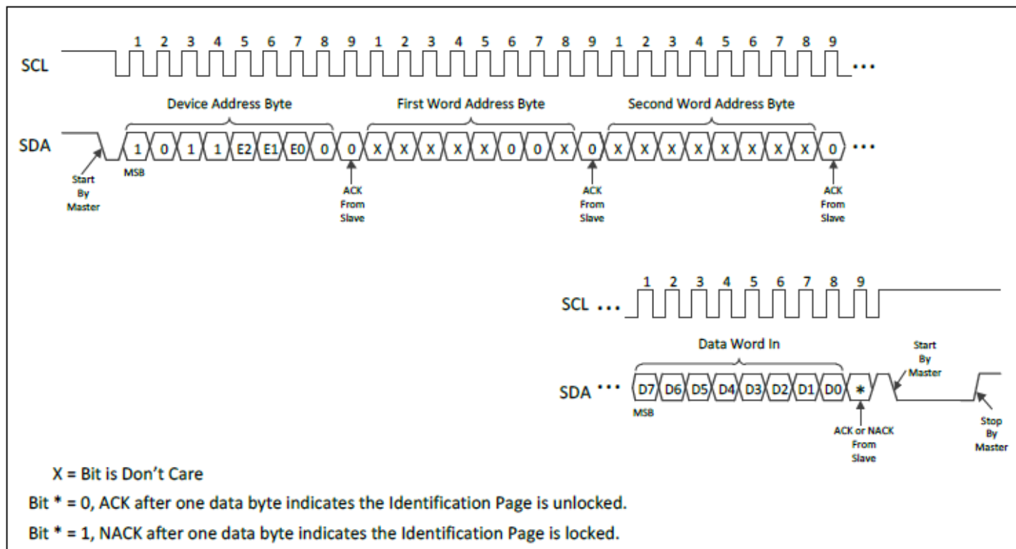
Figure 5–14 Read Lock Status
