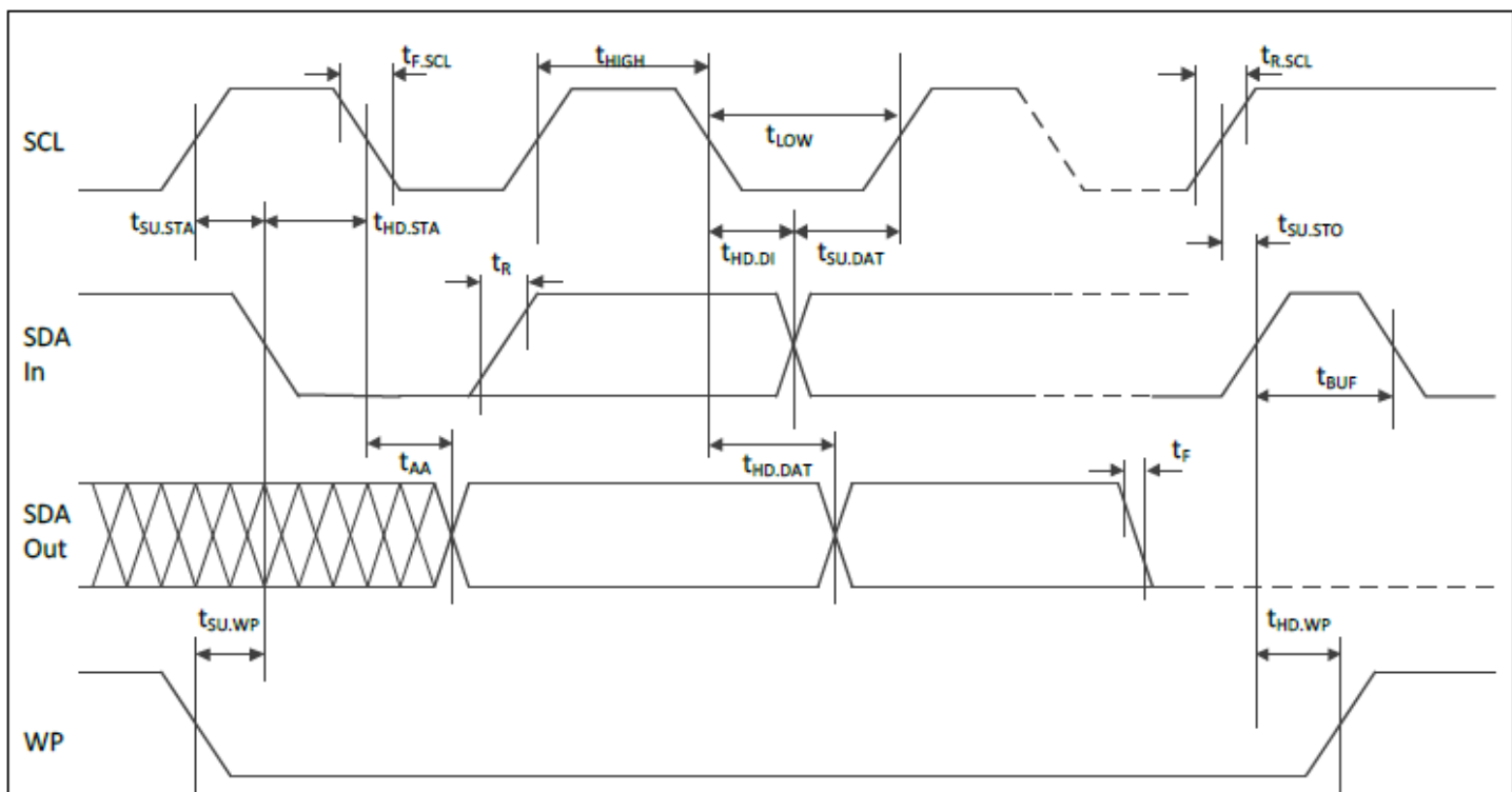
Figure 6–1 Bus Timing
