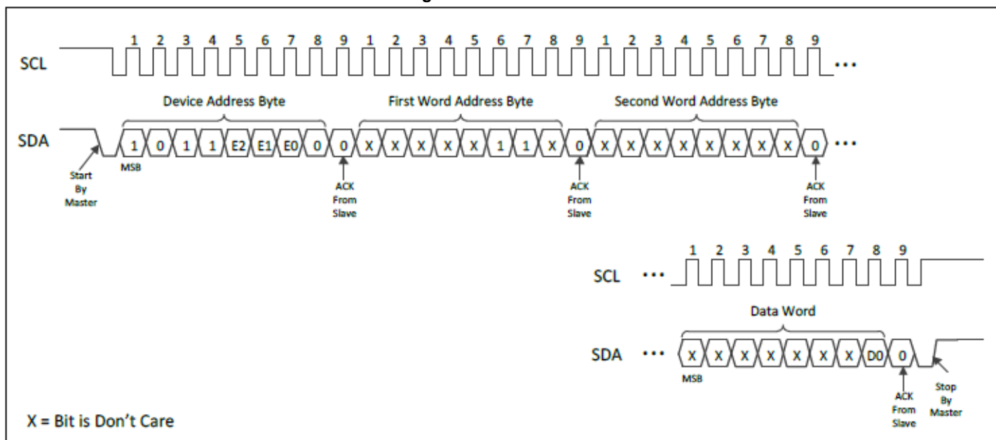
Figure 5–9 Write SWP Bit
