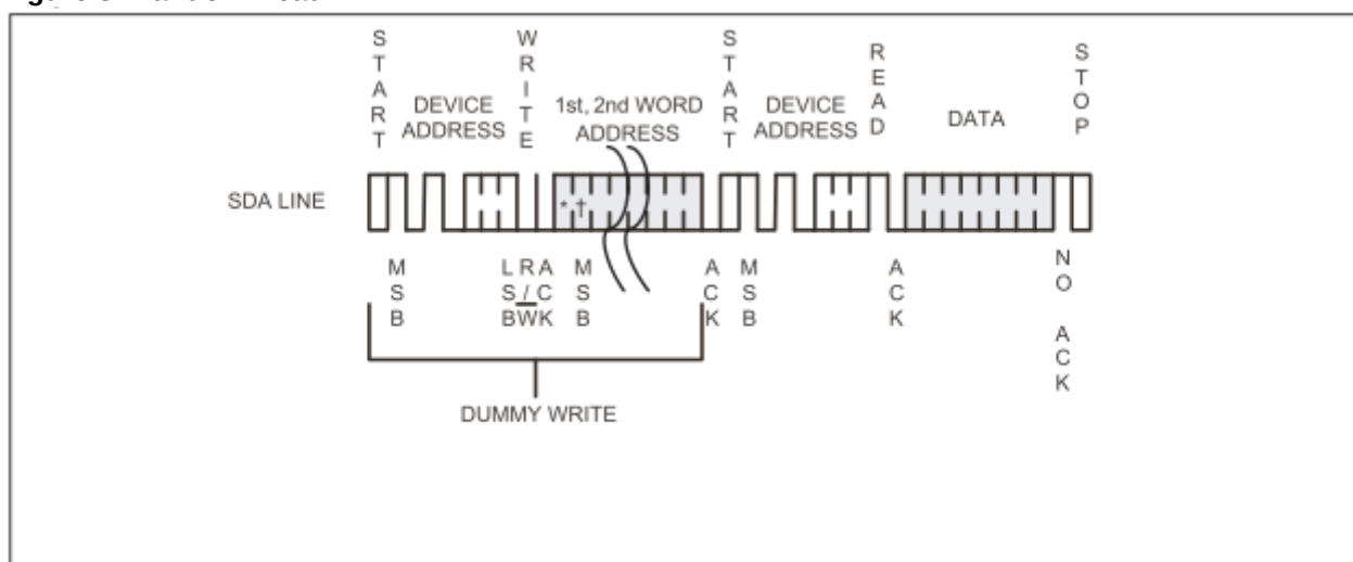
Figure 8: Random Read
