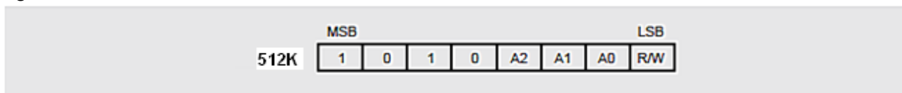
Figure 4: Device Address
