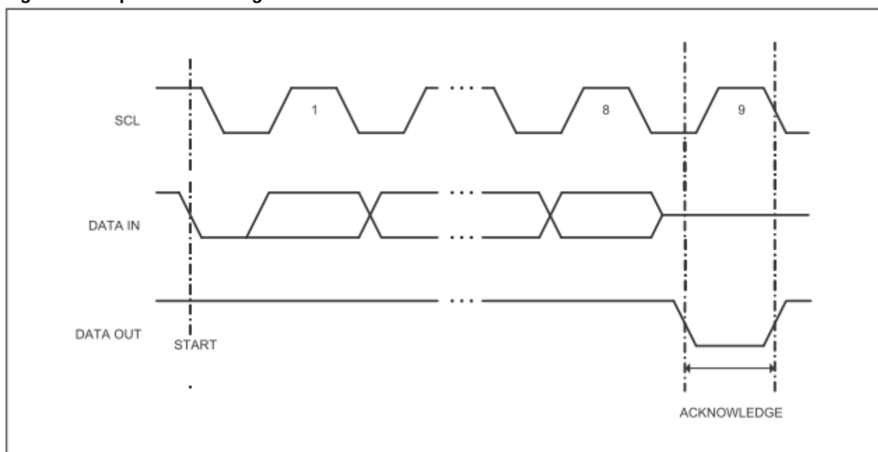
Figure 3: Output Acknowledge
