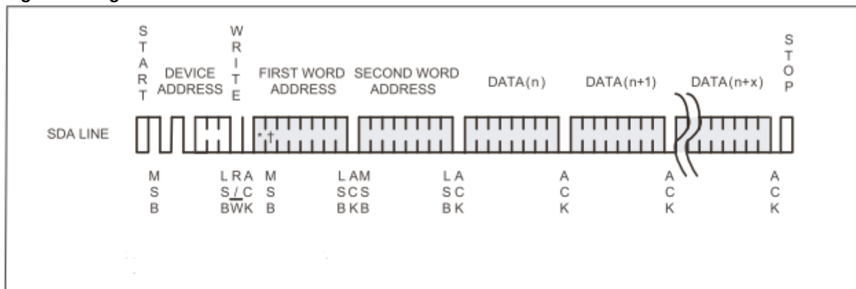
Figure 6: Page Write
