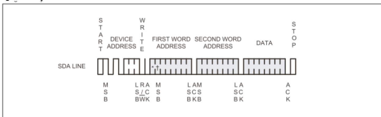
Figure 5: Byte Write
