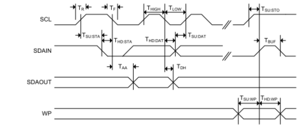
Figure 11 .Bus Timing
