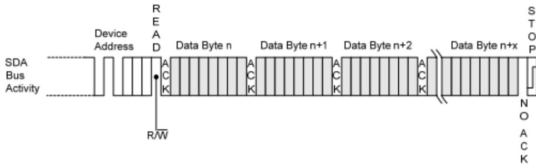
Figure 10. Sequential Read
