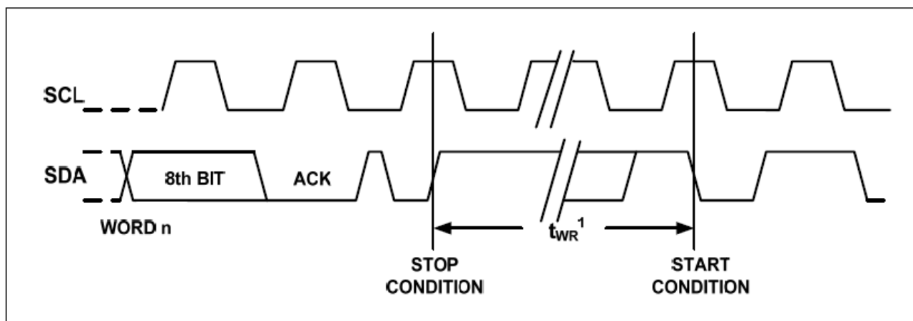
Figure 3 · SCL: Serial Clock, SDA: Serial Data I/O
